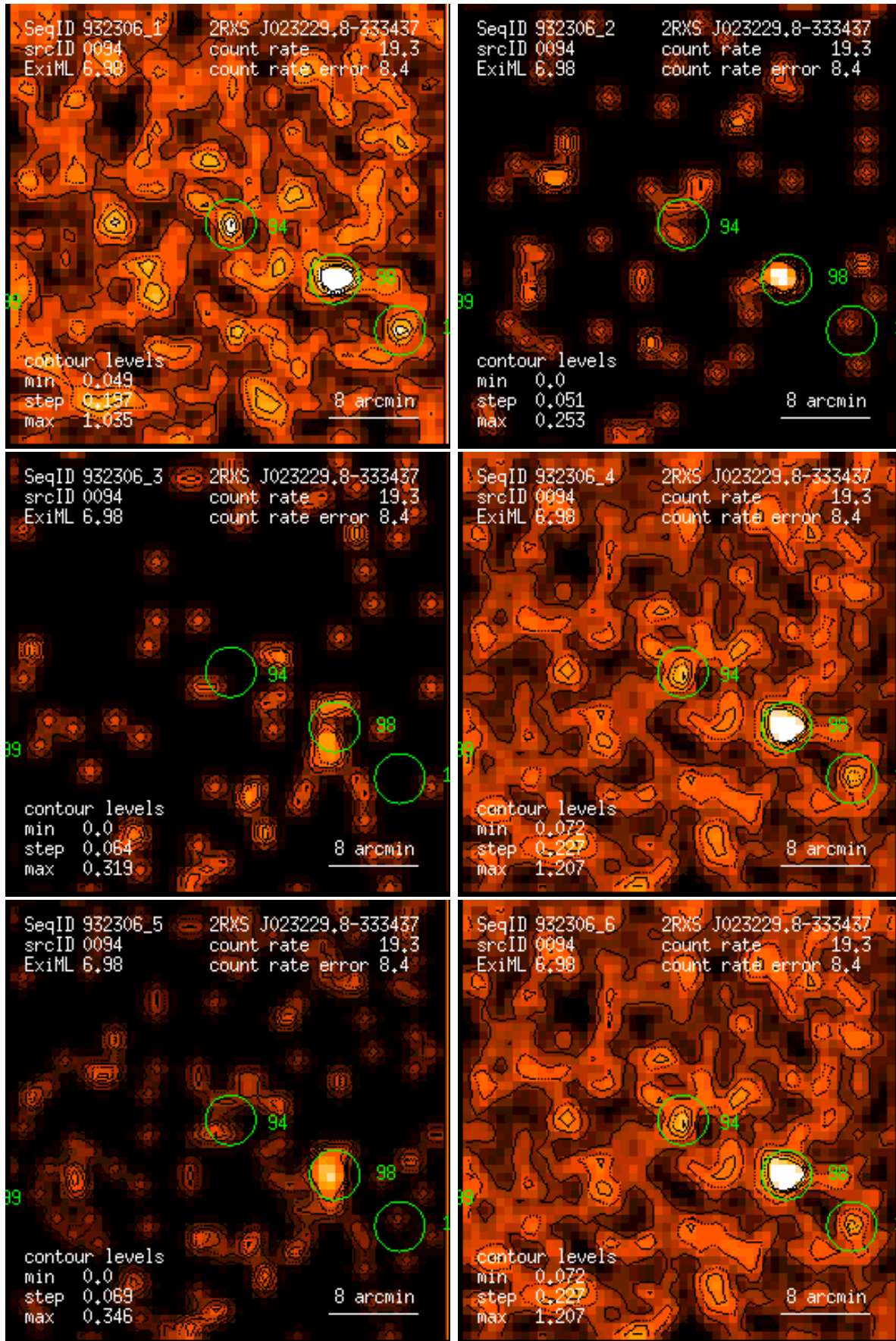
Figure 94: RASS 932306: detection 0094: band rate images, Gaussian filter: (1) PSPC channels 11 – 41, (2) 52 – 90, (3) 91 – 201, (4) 11 – 235, (5) 52 – 201, (6) 11 – 201. Broad band rates in counts/ks. Band rate contour levels in counts/ks/arcmin 2 .
