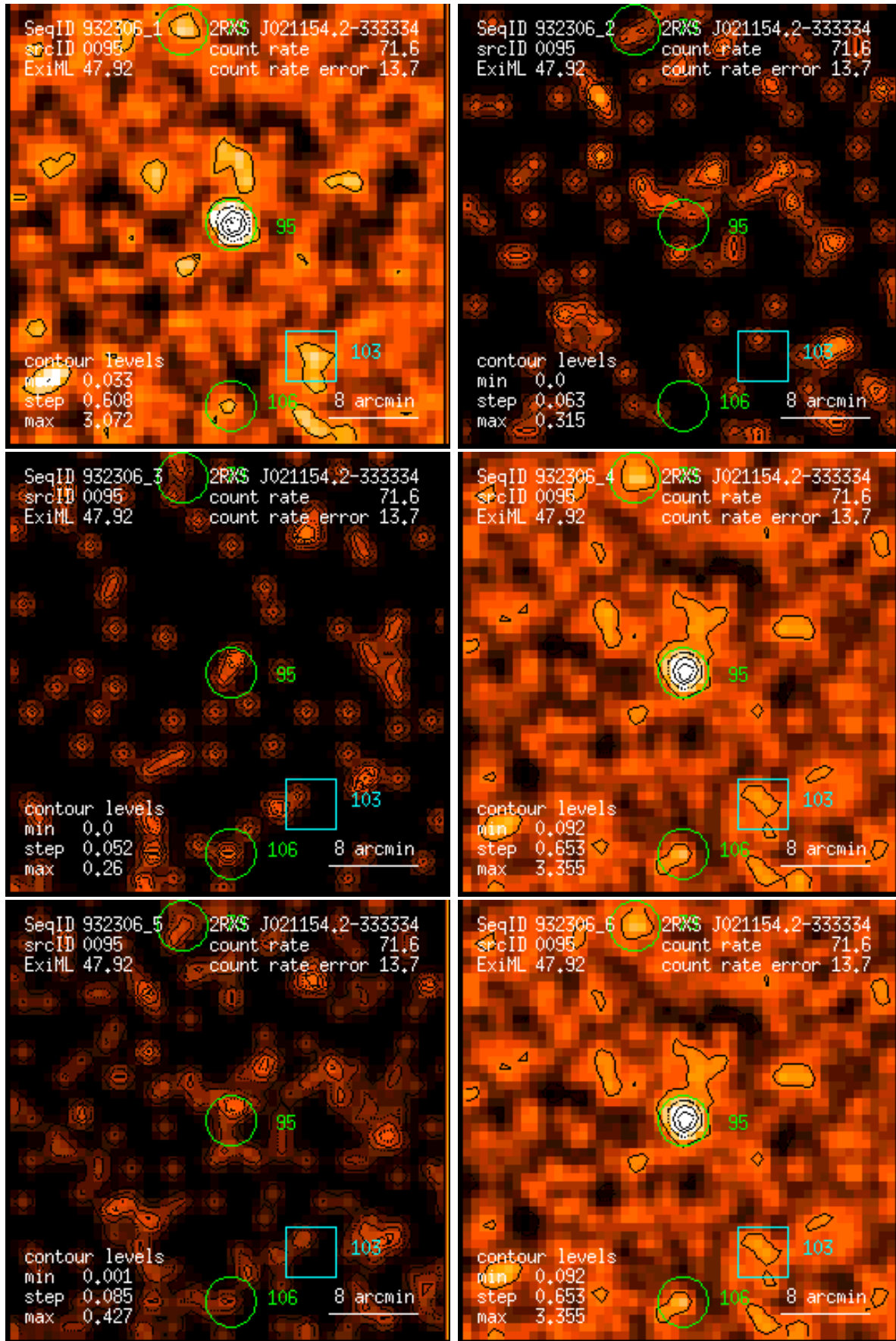
Figure 95: RASS 932306: detection 0095: band rate images, Gaussian filter: (1) PSPC channels 11 – 41, (2) 52 – 90, (3) 91 – 201, (4) 11 – 235, (5) 52 – 201, (6) 11 – 201. Broad band rates in counts/ks. Band rate contour levels in counts/ks/arcmin 2 .
