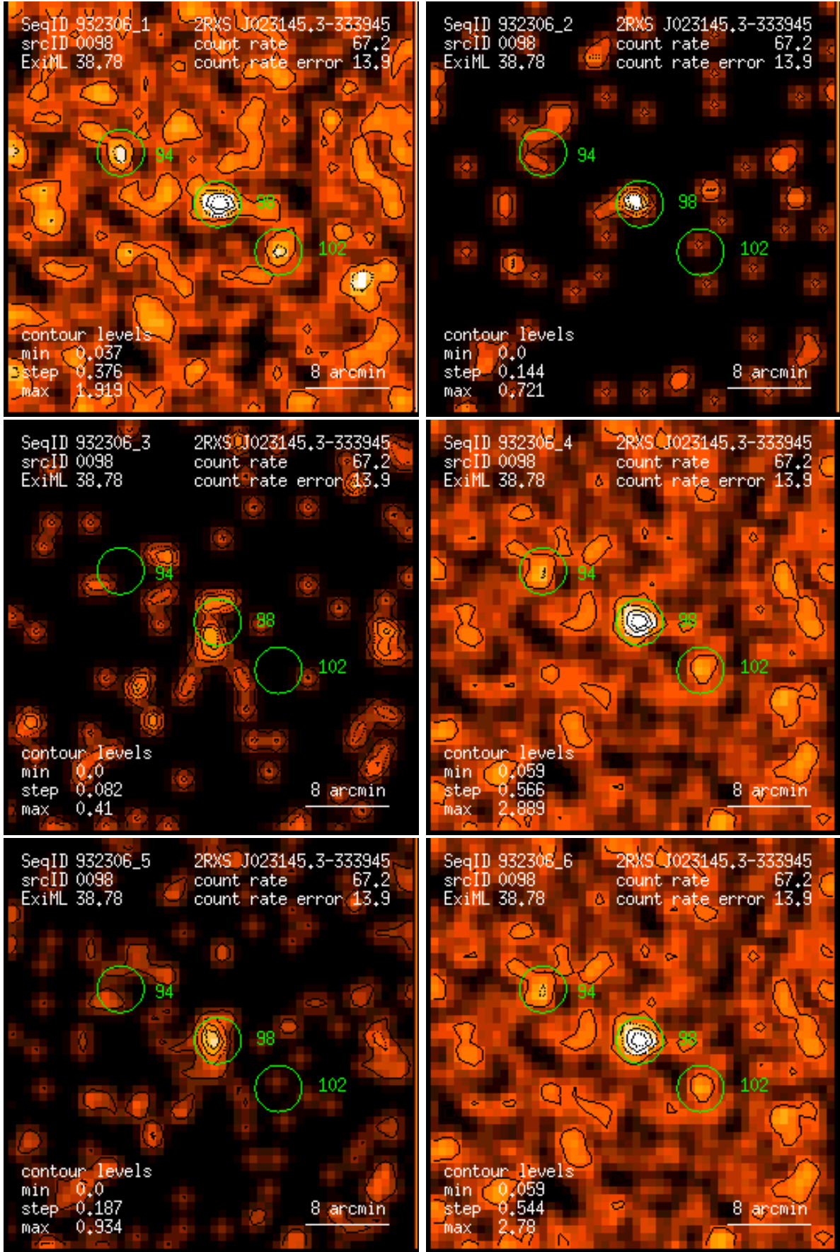
Figure 98: RASS 932306: detection 0098: band rate images, Gaussian filter: (1) PSPC channels 11 – 41, (2) 52 – 90, (3) 91 – 201, (4) 11 – 235, (5) 52 – 201, (6) 11 – 201. Broad band rates in counts/ks. Band rate contour levels in counts/ks/arcmin 2 .
