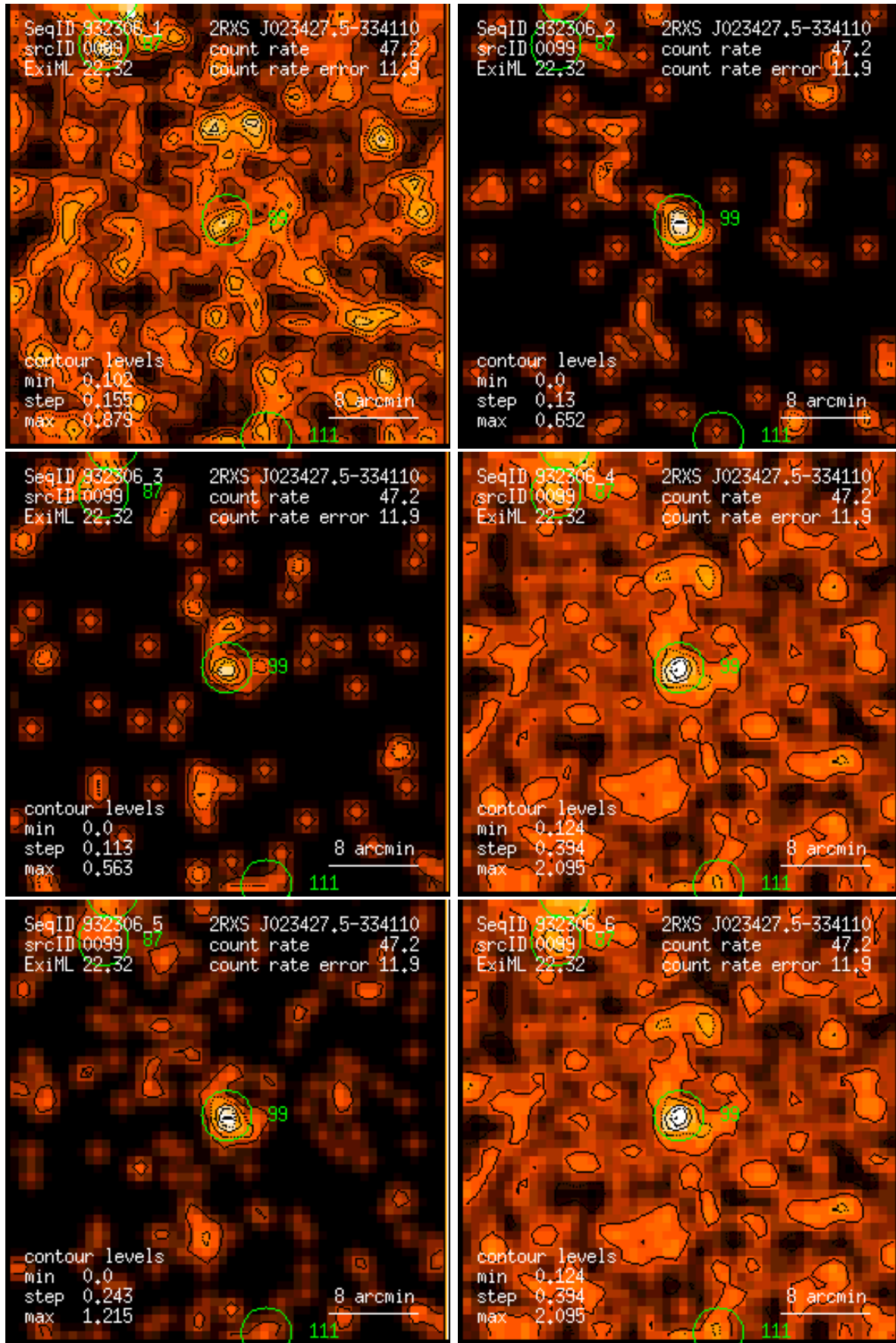
Figure 99: RASS 932306: detection 0099: band rate images, Gaussian filter: (1) PSPC channels 11 – 41, (2) 52 – 90, (3) 91 – 201, (4) 11 – 235, (5) 52 – 201, (6) 11 – 201. Broad band rates in counts/ks. Band rate contour levels in counts/ks/arcmin 2 .
