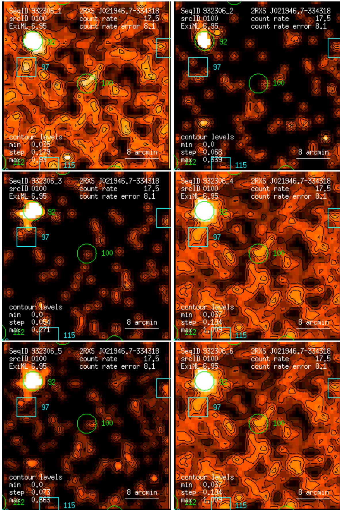
Figure 100: RASS 932306: detection 0100: band rate images, Gaussian filter: (1) PSPC channels 11 – 41, (2) 52 – 90, (3) 91 – 201, (4) 11 – 235, (5) 52 – 201, (6) 11 – 201. Broad band rates in counts/ks. Band rate contour levels in counts/ks/arcmin 2 .
