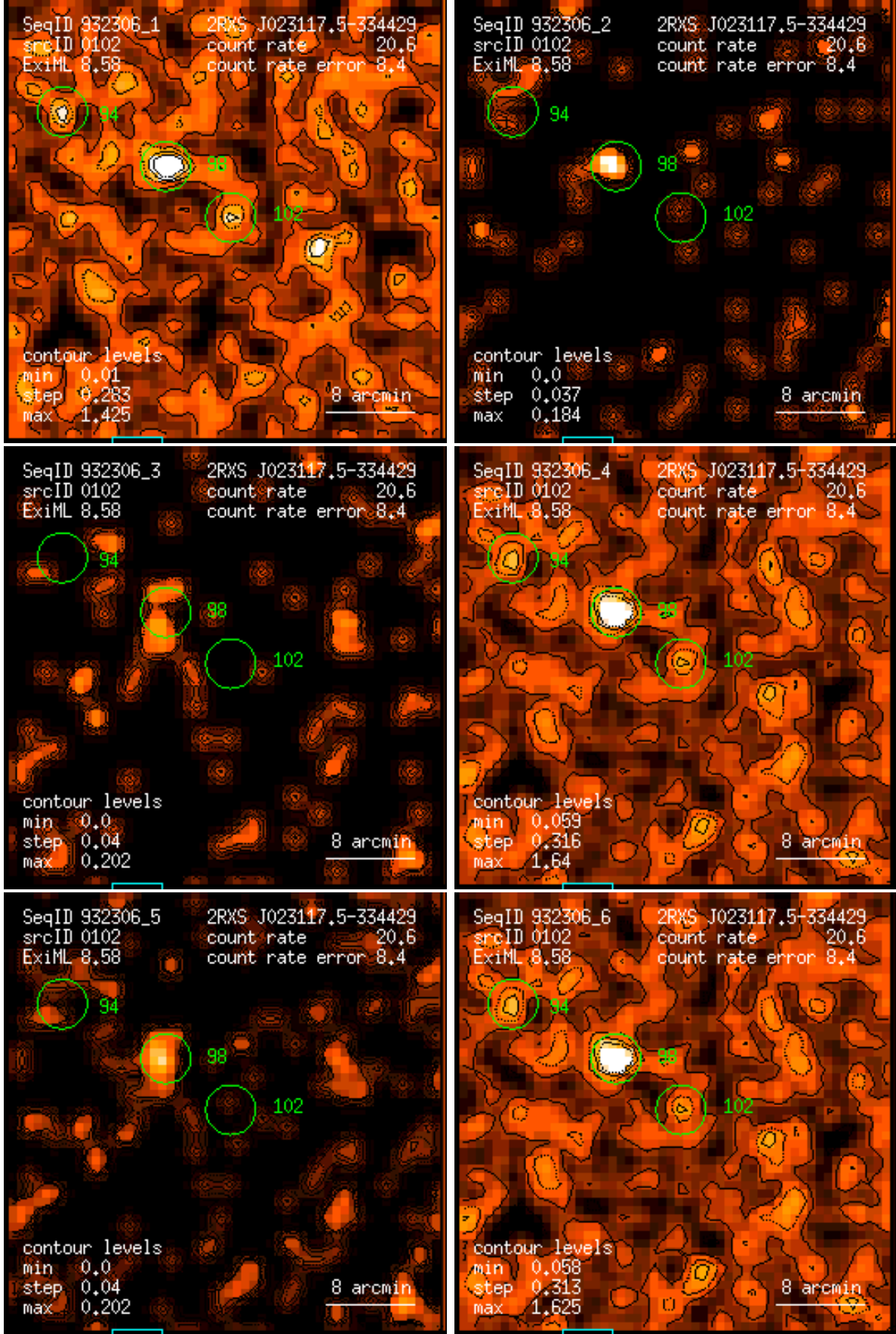
Figure 102: RASS 932306: detection 0102: band rate images, Gaussian filter: (1) PSPC channels 11 – 41, (2) 52 – 90, (3) 91 – 201, (4) 11 – 235, (5) 52 – 201, (6) 11 – 201. Broad band rates in counts/ks. Band rate contour levels in counts/ks/arcmin 2 .
