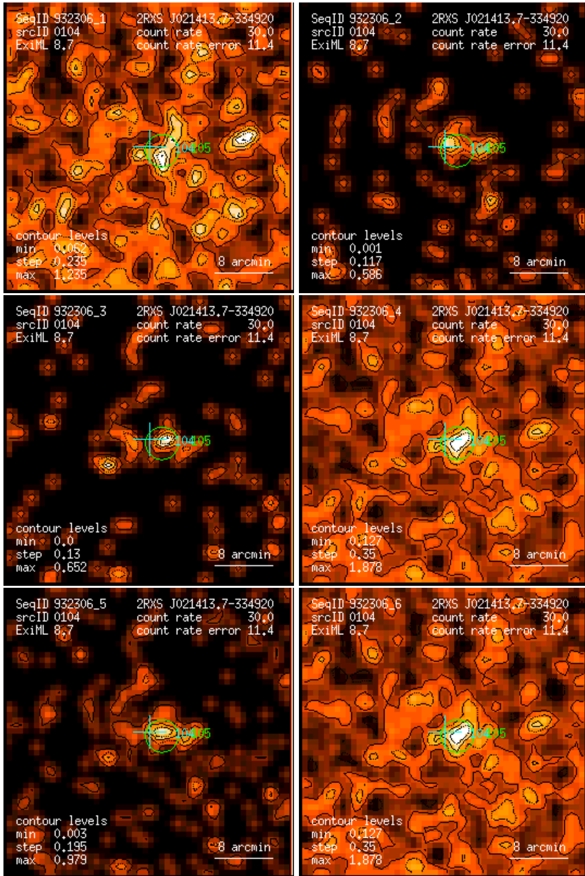
Figure 104: RASS 932306: detection 0104: band rate images, Gaussian filter: (1) PSPC channels 11 – 41, (2) 52 – 90, (3) 91 – 201, (4) 11 – 235, (5) 52 – 201, (6) 11 – 201. Broad band rates in counts/ks. Band rate contour levels in counts/ks/arcmin 2 .
