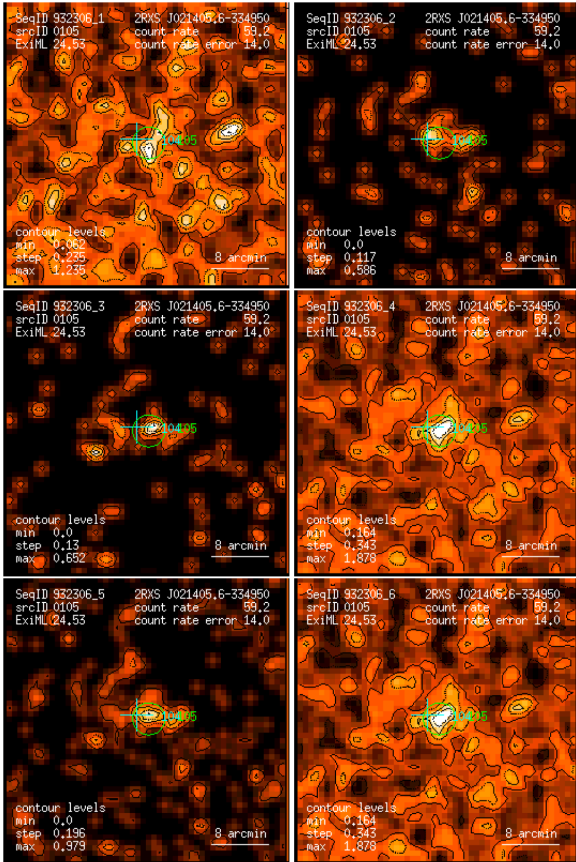
Figure 105: RASS 932306: detection 0105: band rate images, Gaussian filter: (1) PSPC channels 11 – 41, (2) 52 – 90, (3) 91 – 201, (4) 11 – 235, (5) 52 – 201, (6) 11 – 201. Broad band rates in counts/ks. Band rate contour levels in counts/ks/arcmin 2 .
