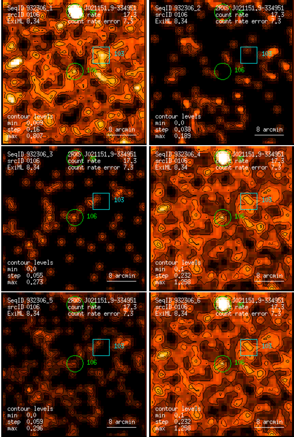
Figure 106: RASS 932306: detection 0106: band rate images, Gaussian filter: (1) PSPC channels 11 – 41, (2) 52 – 90, (3) 91 – 201, (4) 11 – 235, (5) 52 – 201, (6) 11 – 201. Broad band rates in counts/ks. Band rate contour levels in counts/ks/arcmin 2 .
