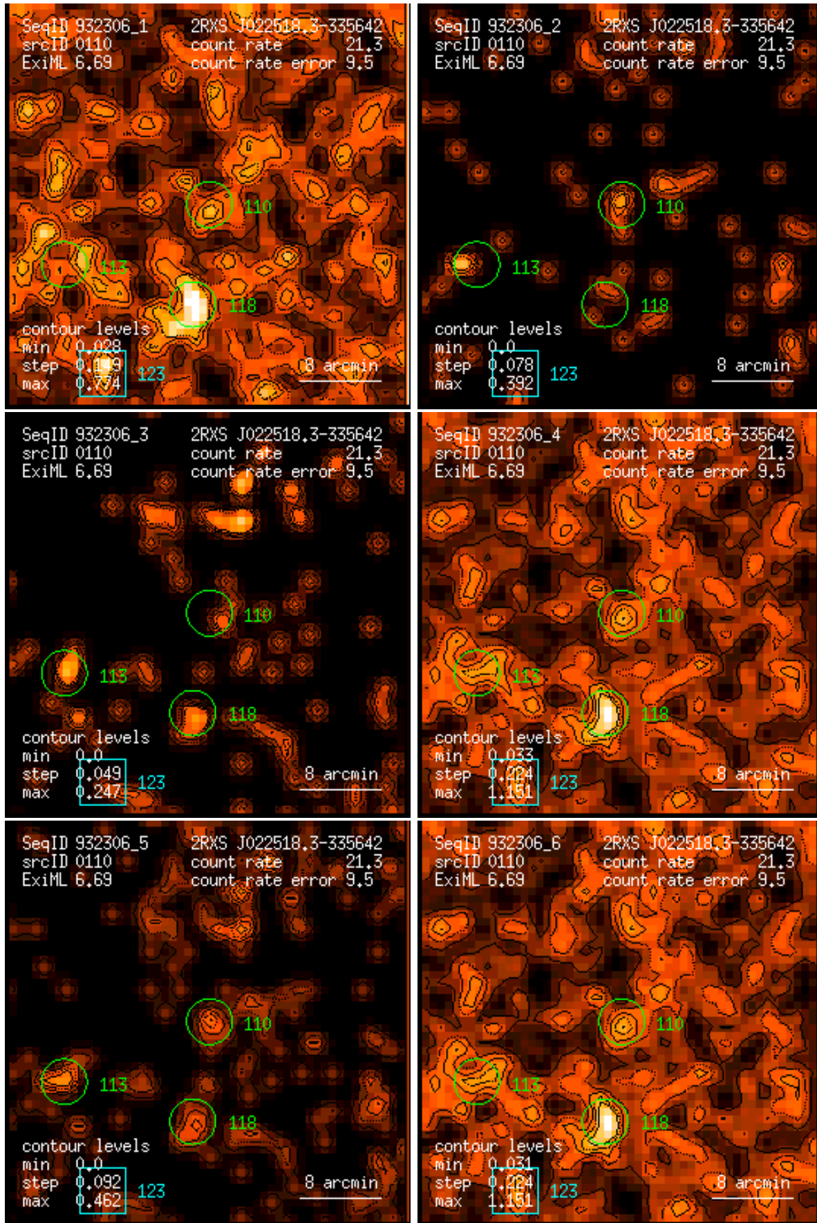
Figure 110: RASS 932306: detection 0110: band rate images, Gaussian filter: (1) PSPC channels 11 – 41, (2) 52 – 90, (3) 91 – 201, (4) 11 – 235, (5) 52 – 201, (6) 11 – 201. Broad band rates in counts/ks. Band rate contour levels in counts/ks/arcmin 2 .
