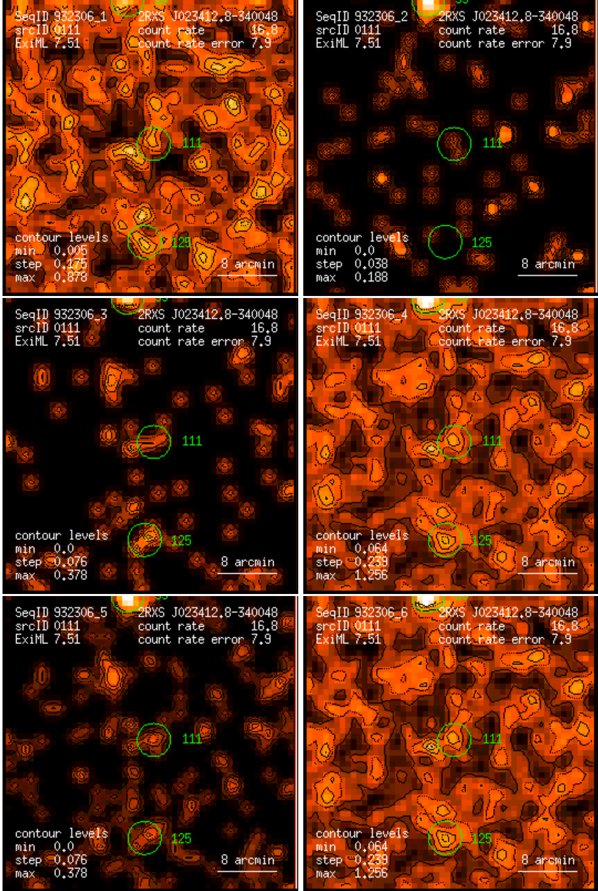
Figure 111: RASS 932306: detection 0111: band rate images, Gaussian filter: (1) PSPC channels 11 – 41, (2) 52 – 90, (3) 91 – 201, (4) 11 – 235, (5) 52 – 201, (6) 11 – 201. Broad band rates in counts/ks. Band rate contour levels in counts/ks/arcmin 2 .
