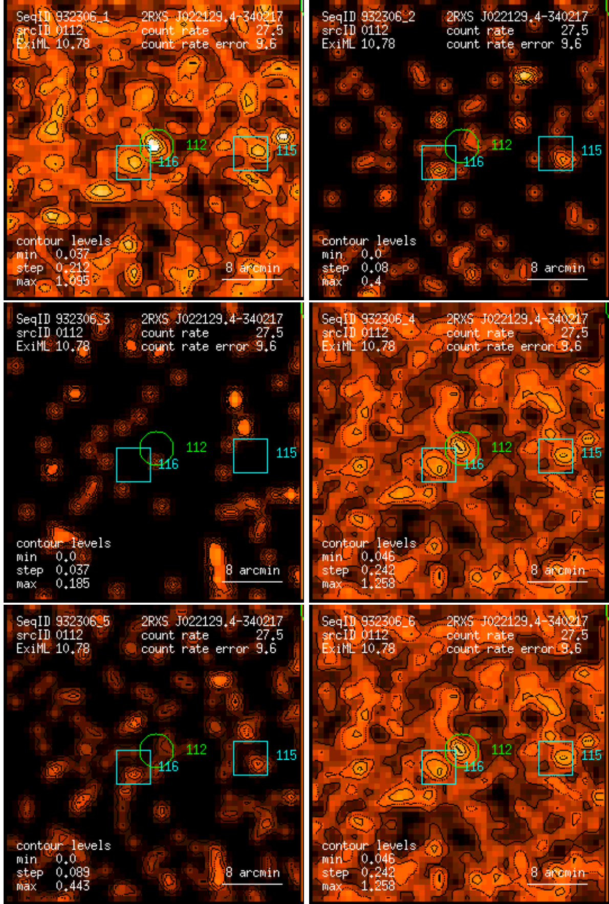
Figure 112: RASS 932306: detection 0112: band rate images, Gaussian filter: (1) PSPC channels 11 – 41, (2) 52 – 90, (3) 91 – 201, (4) 11 – 235, (5) 52 – 201, (6) 11 – 201. Broad band rates in counts/ks. Band rate contour levels in counts/ks/arcmin 2 .
