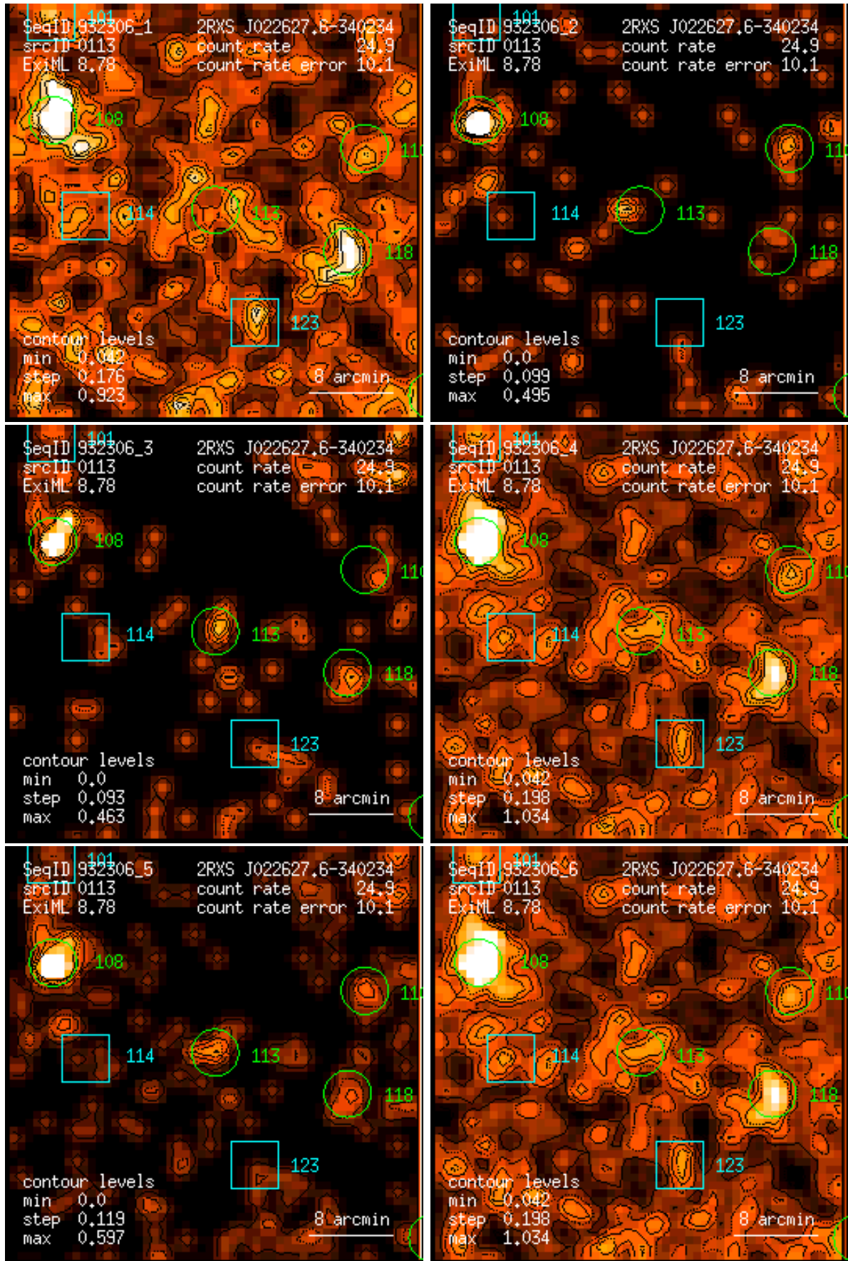
Figure 113: RASS 932306: detection 0113: band rate images, Gaussian filter: (1) PSPC channels 11 – 41, (2) 52 – 90, (3) 91 – 201, (4) 11 – 235, (5) 52 – 201, (6) 11 – 201. Broad band rates in counts/ks. Band rate contour levels in counts/ks/arcmin 2 .
