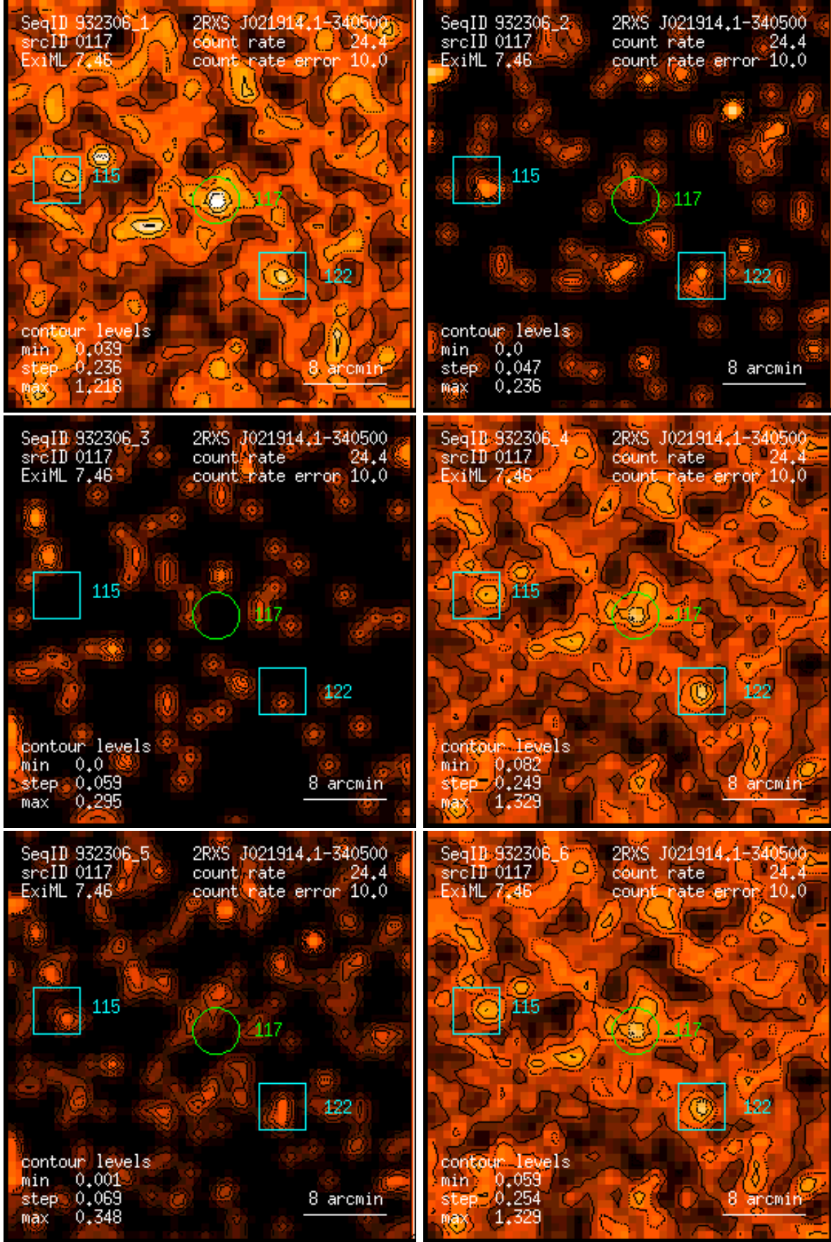
Figure 117: RASS 932306: detection 0117: band rate images, Gaussian filter: (1) PSPC channels 11 – 41, (2) 52 – 90, (3) 91 – 201, (4) 11 – 235, (5) 52 – 201, (6) 11 – 201. Broad band rates in counts/ks. Band rate contour levels in counts/ks/arcmin 2 .
