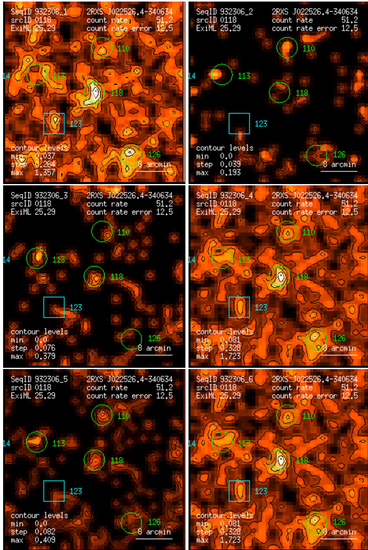
Figure 118: RASS 932306: detection 0118: band rate images, Gaussian filter: (1) PSPC channels 11 – 41, (2) 52 – 90, (3) 91 – 201, (4) 11 – 235, (5) 52 – 201, (6) 11 – 201. Broad band rates in counts/ks. Band rate contour levels in counts/ks/arcmin 2 .
