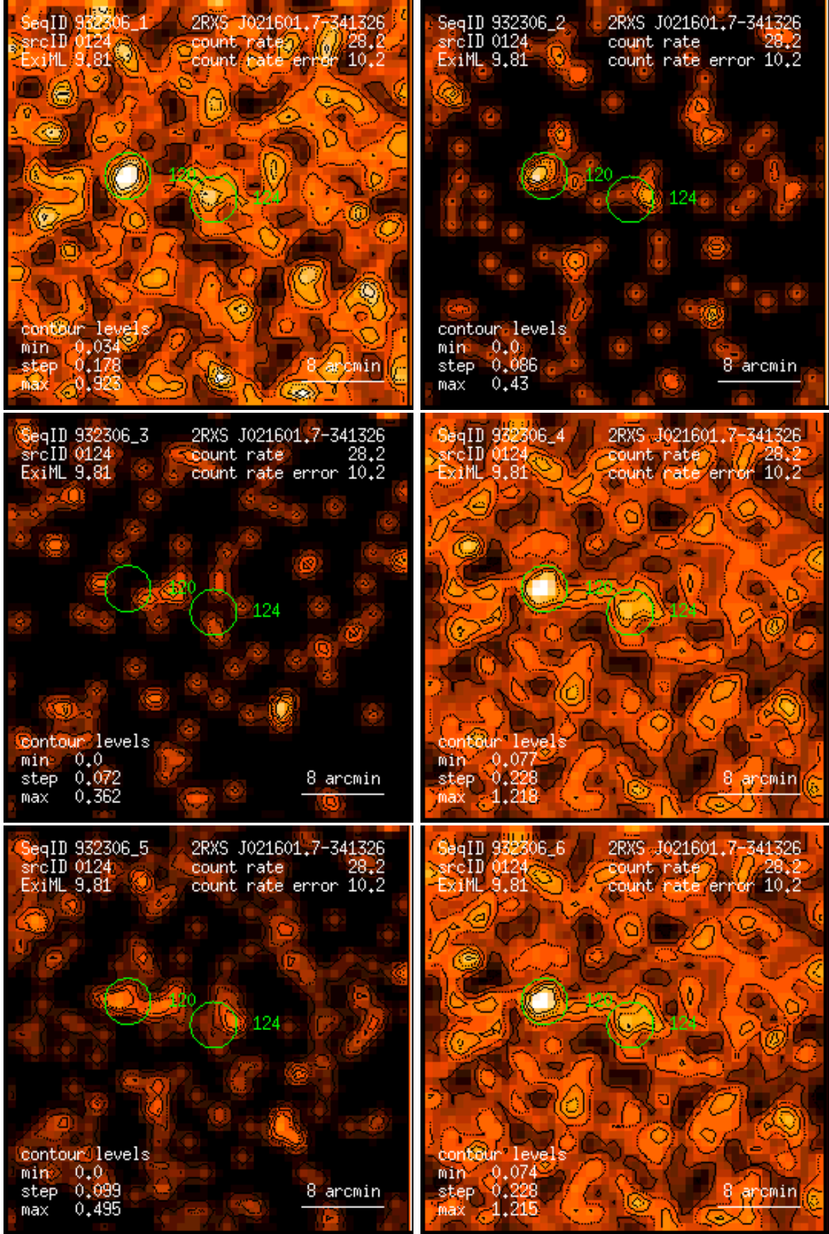
Figure 124: RASS 932306: detection 0124: band rate images, Gaussian filter: (1) PSPC channels 11 – 41, (2) 52 – 90, (3) 91 – 201, (4) 11 – 235, (5) 52 – 201, (6) 11 – 201. Broad band rates in counts/ks. Band rate contour levels in counts/ks/arcmin 2 .
