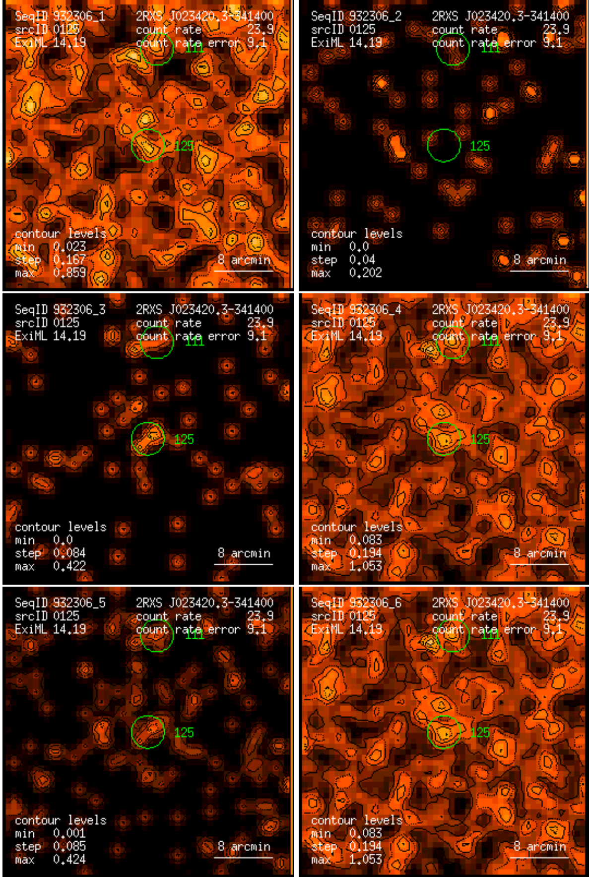
Figure 125: RASS 932306: detection 0125: band rate images, Gaussian filter: (1) PSPC channels 11 – 41, (2) 52 – 90, (3) 91 – 201, (4) 11 – 235, (5) 52 – 201, (6) 11 – 201. Broad band rates in counts/ks. Band rate contour levels in counts/ks/arcmin 2 .
