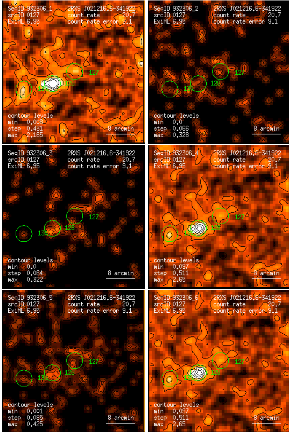
Figure 127: RASS 932306: detection 0127: band rate images, Gaussian filter: (1) PSPC channels 11 – 41, (2) 52 – 90, (3) 91 – 201, (4) 11 – 235, (5) 52 – 201, (6) 11 – 201. Broad band rates in counts/ks. Band rate contour levels in counts/ks/arcmin 2 .
