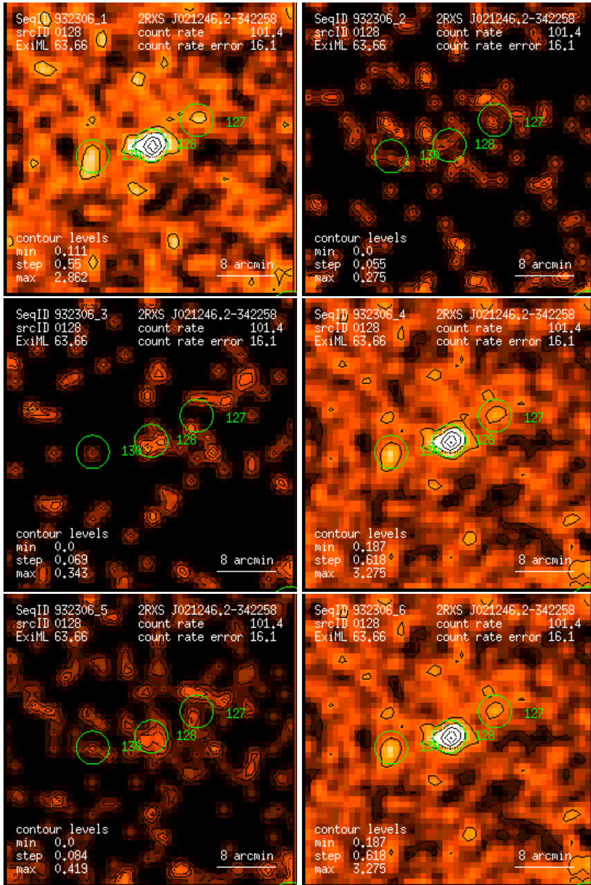
Figure 128: RASS 932306: detection 0128: band rate images, Gaussian filter: (1) PSPC channels 11 – 41, (2) 52 – 90, (3) 91 – 201, (4) 11 – 235, (5) 52 – 201, (6) 11 – 201. Broad band rates in counts/ks. Band rate contour levels in counts/ks/arcmin 2 .
