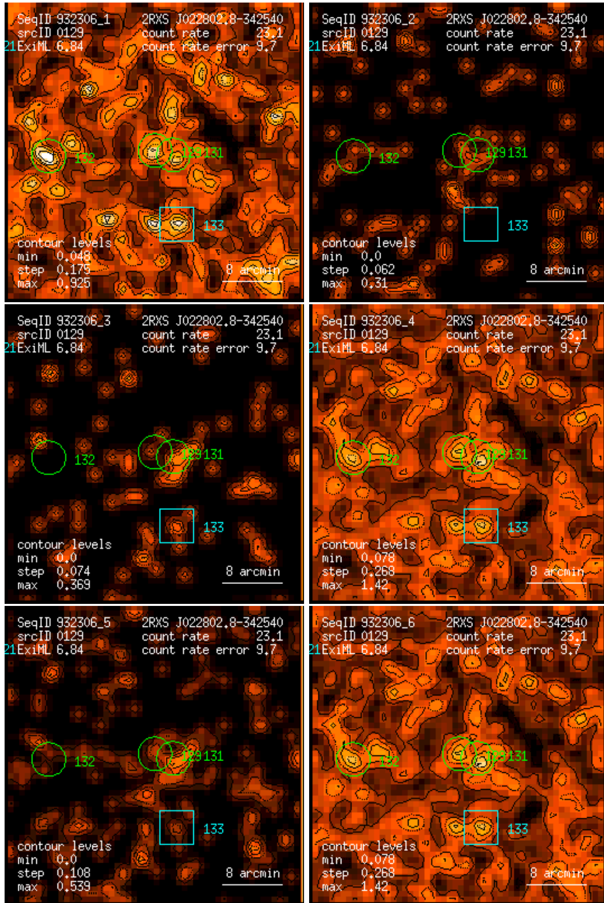
Figure 129: RASS 932306: detection 0129: band rate images, Gaussian filter: (1) PSPC channels 11 – 41, (2) 52 – 90, (3) 91 – 201, (4) 11 – 235, (5) 52 – 201, (6) 11 – 201. Broad band rates in counts/ks. Band rate contour levels in counts/ks/arcmin 2 .
