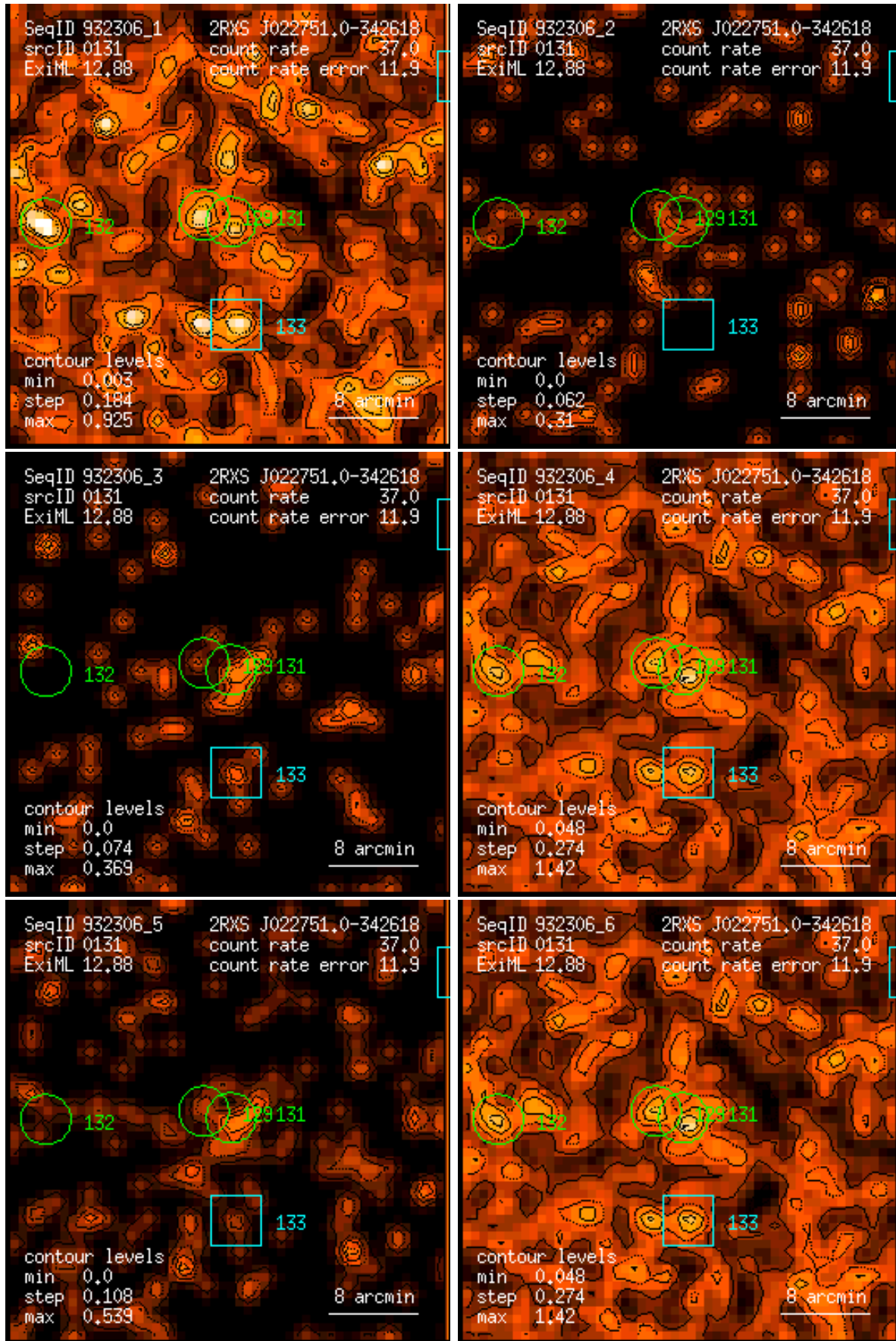
Figure 131: RASS 932306: detection 0131: band rate images, Gaussian filter: (1) PSPC channels 11 – 41, (2) 52 – 90, (3) 91 – 201, (4) 11 – 235, (5) 52 – 201, (6) 11 – 201. Broad band rates in counts/ks. Band rate contour levels in counts/ks/arcmin 2 .
