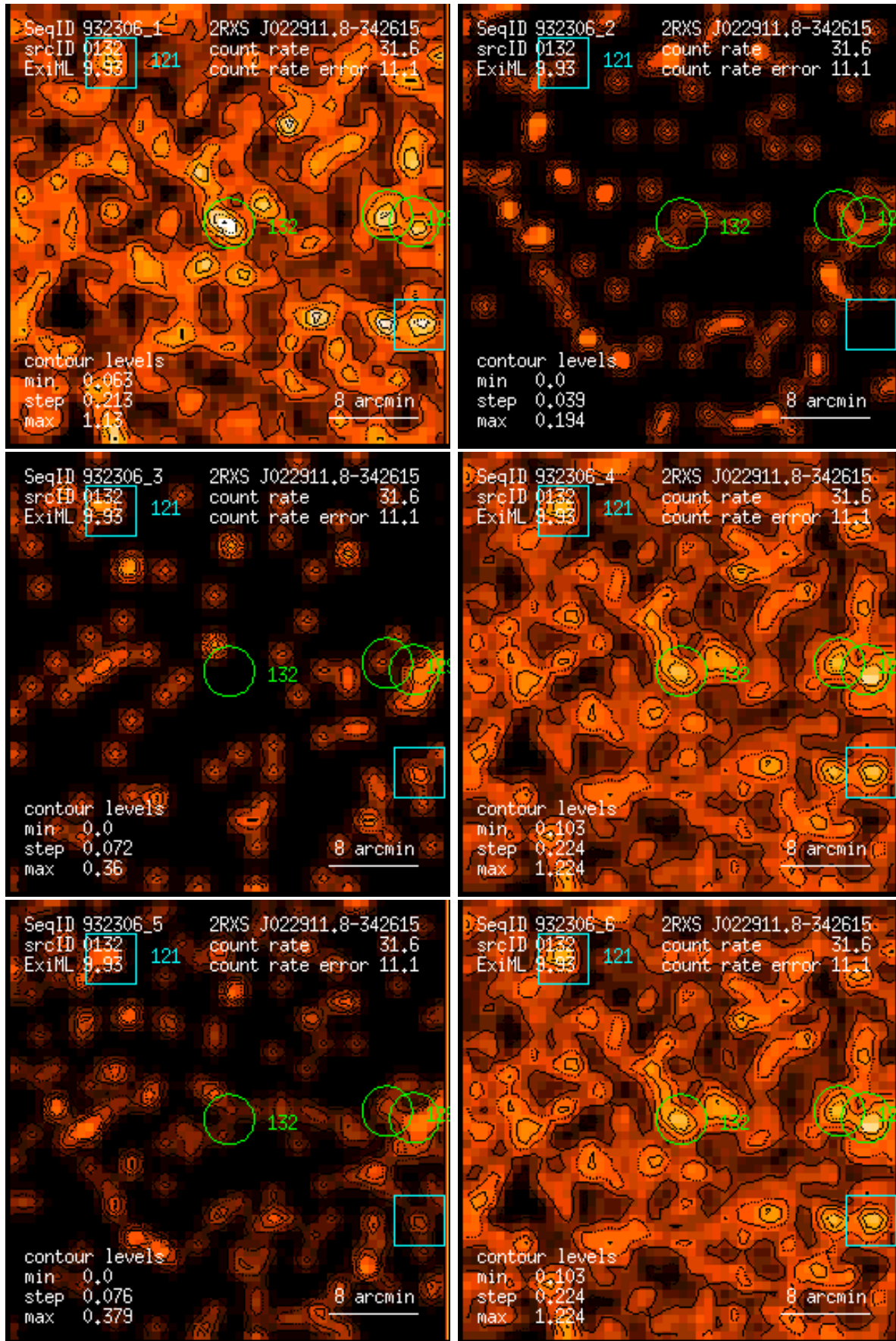
Figure 132: RASS 932306: detection 0132: band rate images, Gaussian filter: (1) PSPC channels 11 – 41, (2) 52 – 90, (3) 91 – 201, (4) 11 – 235, (5) 52 – 201, (6) 11 – 201. Broad band rates in counts/ks. Band rate contour levels in counts/ks/arcmin 2 .
