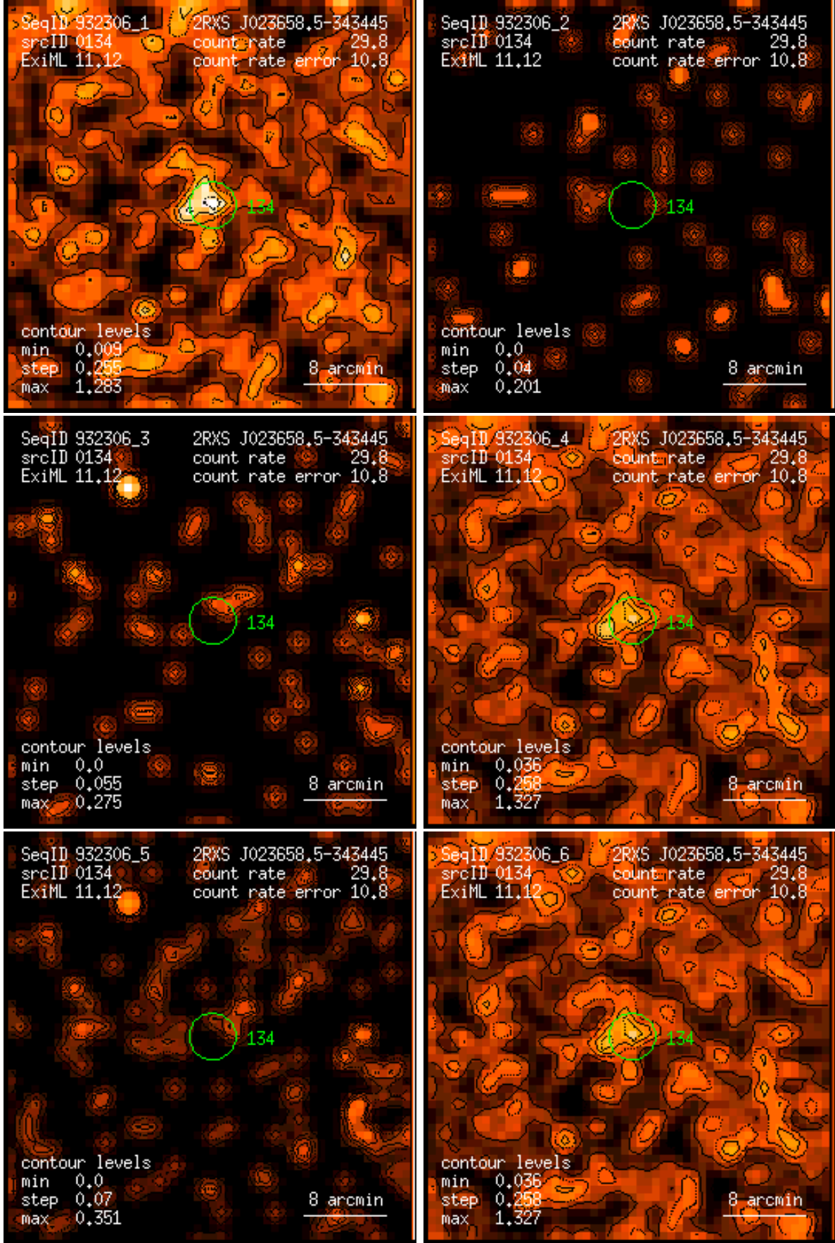
Figure 134: RASS 932306: detection 0134: band rate images, Gaussian filter: (1) PSPC channels 11 – 41, (2) 52 – 90, (3) 91 – 201, (4) 11 – 235, (5) 52 – 201, (6) 11 – 201. Broad band rates in counts/ks. Band rate contour levels in counts/ks/arcmin 2 .
