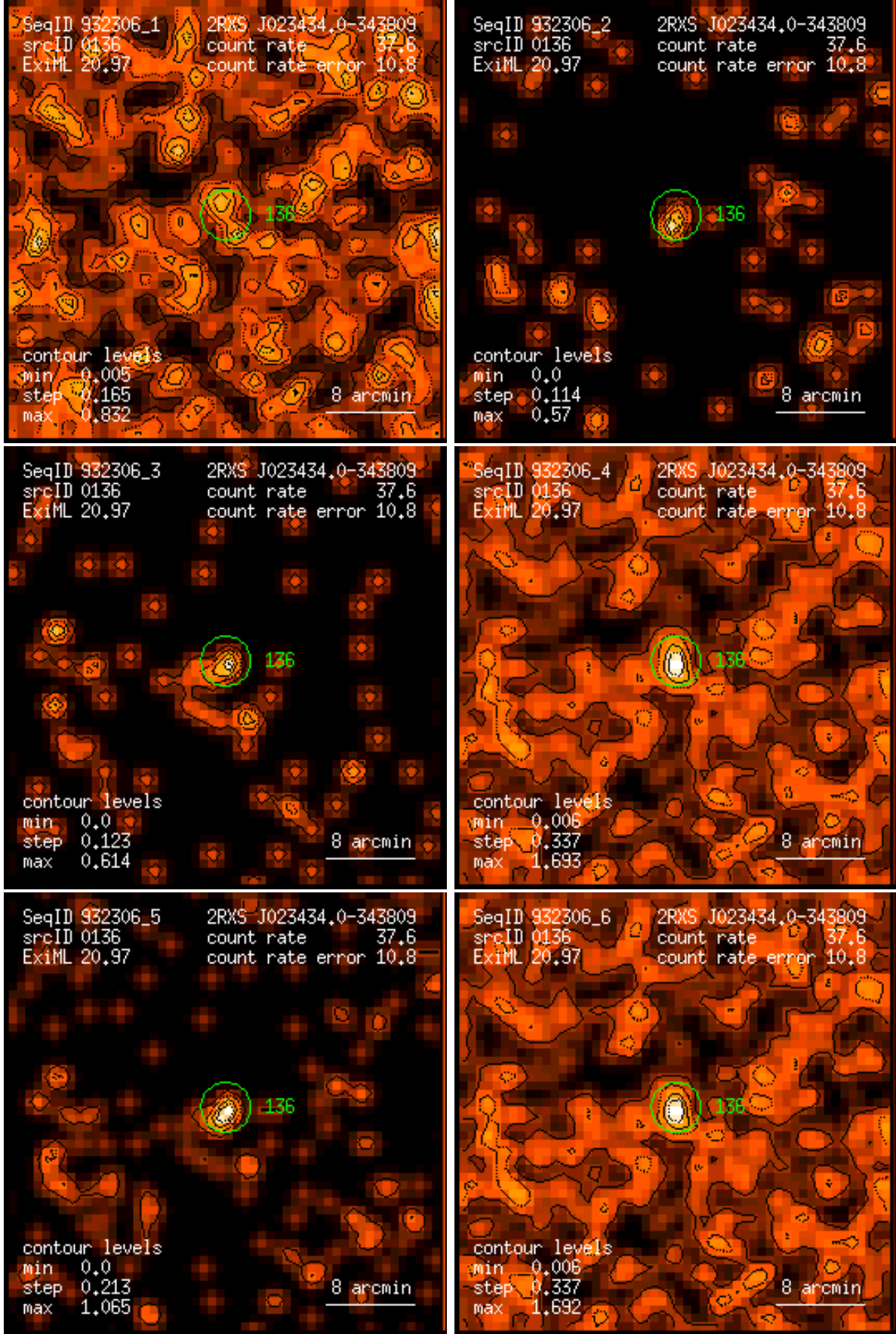
Figure 136: RASS 932306: detection 0136: band rate images, Gaussian filter: (1) PSPC channels 11 – 41, (2) 52 – 90, (3) 91 – 201, (4) 11 – 235, (5) 52 – 201, (6) 11 – 201. Broad band rates in counts/ks. Band rate contour levels in counts/ks/arcmin 2 .
