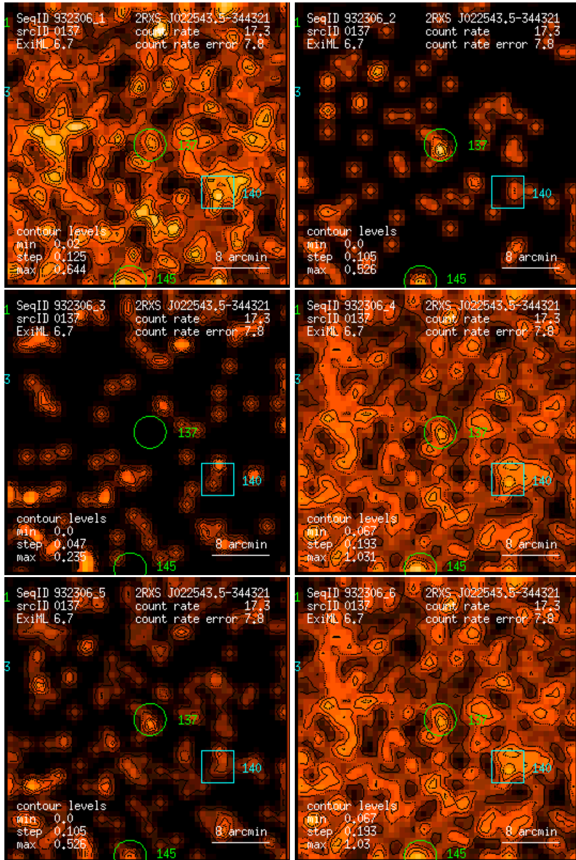
Figure 137: RASS 932306: detection 0137: band rate images, Gaussian filter: (1) PSPC channels 11 – 41, (2) 52 – 90, (3) 91 – 201, (4) 11 – 235, (5) 52 – 201, (6) 11 – 201. Broad band rates in counts/ks. Band rate contour levels in counts/ks/arcmin 2 .
