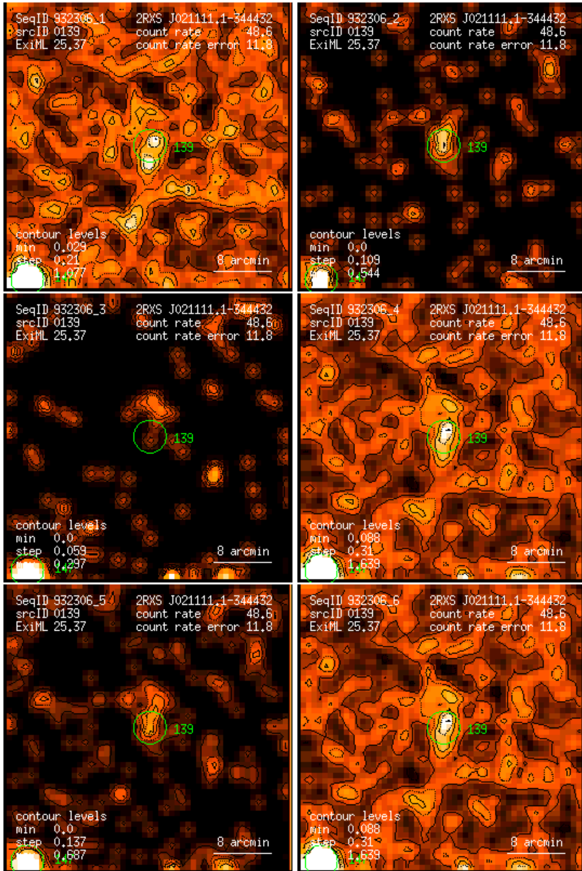
Figure 139: RASS 932306: detection 0139: band rate images, Gaussian filter: (1) PSPC channels 11 – 41, (2) 52 – 90, (3) 91 – 201, (4) 11 – 235, (5) 52 – 201, (6) 11 – 201. Broad band rates in counts/ks. Band rate contour levels in counts/ks/arcmin 2 .
