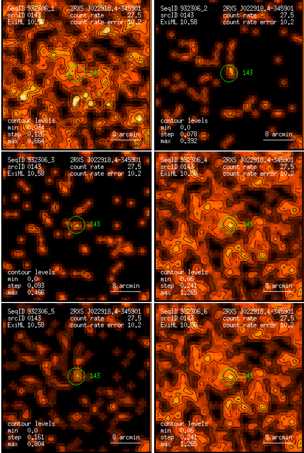
Figure 143: RASS 932306: detection 0143: band rate images, Gaussian filter: (1) PSPC channels 11 – 41, (2) 52 – 90, (3) 91 – 201, (4) 11 – 235, (5) 52 – 201, (6) 11 – 201. Broad band rates in counts/ks. Band rate contour levels in counts/ks/arcmin 2 .
