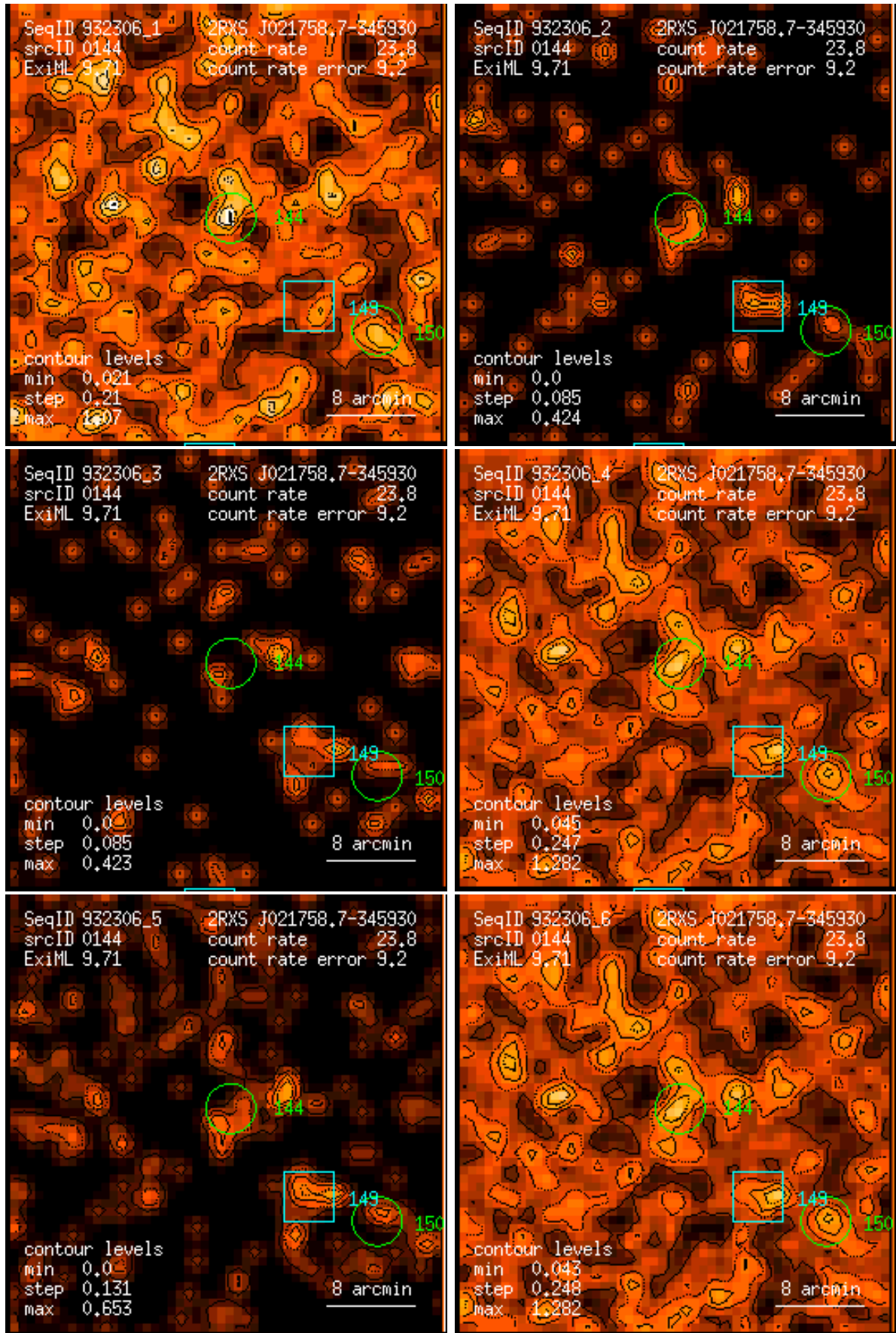
Figure 144: RASS 932306: detection 0144: band rate images, Gaussian filter: (1) PSPC channels 11 – 41, (2) 52 – 90, (3) 91 – 201, (4) 11 – 235, (5) 52 – 201, (6) 11 – 201. Broad band rates in counts/ks. Band rate contour levels in counts/ks/arcmin 2 .
