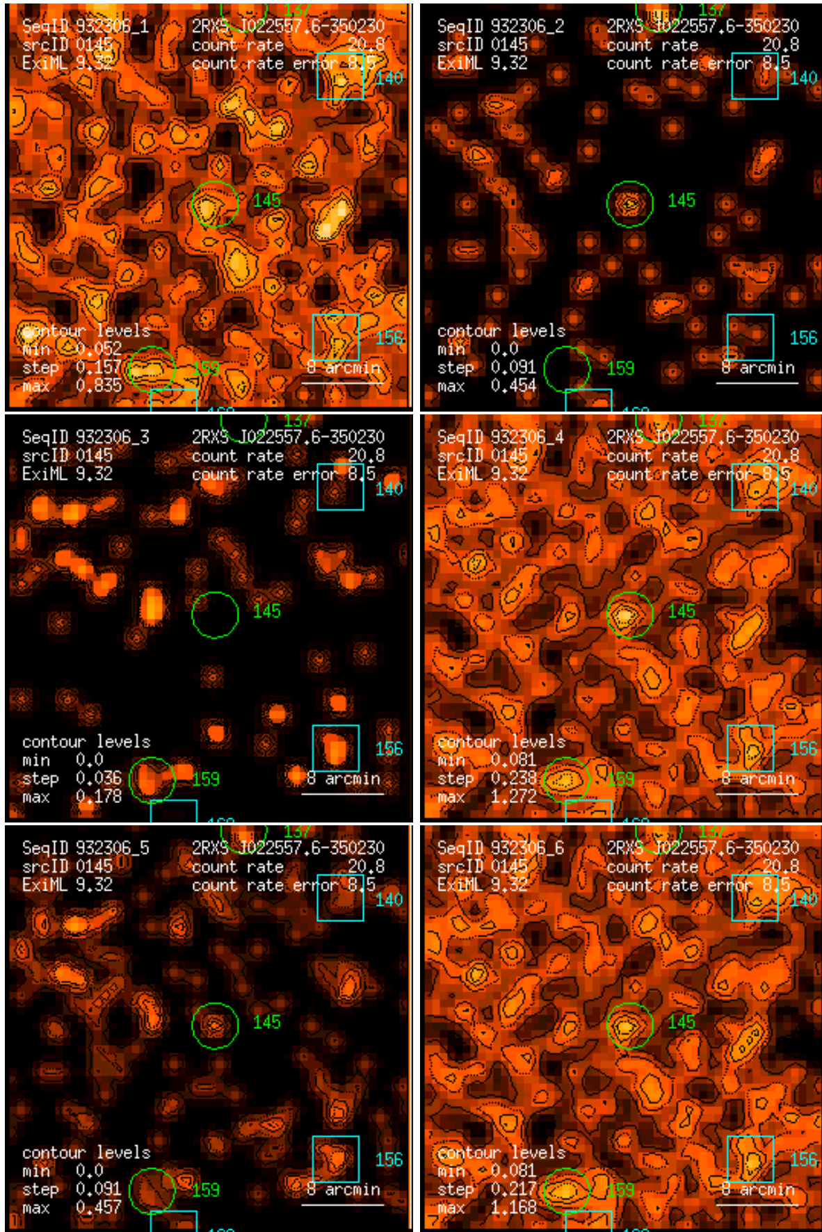
Figure 145: RASS 932306: detection 0145: band rate images, Gaussian filter: (1) PSPC channels 11 – 41, (2) 52 – 90, (3) 91 – 201, (4) 11 – 235, (5) 52 – 201, (6) 11 – 201. Broad band rates in counts/ks. Band rate contour levels in counts/ks/arcmin 2 .
