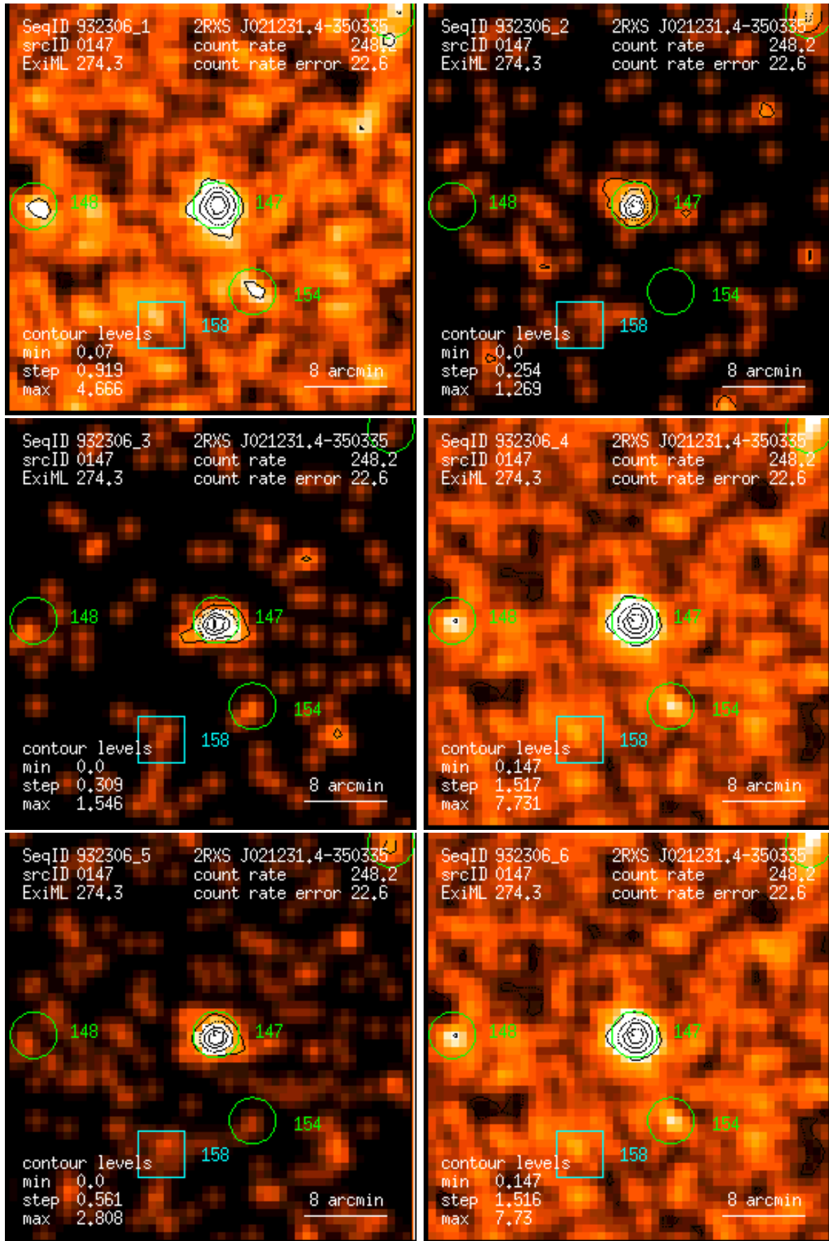
Figure 147: RASS 932306: detection 0147: band rate images, Gaussian filter: (1) PSPC channels 11 – 41, (2) 52 – 90, (3) 91 – 201, (4) 11 – 235, (5) 52 – 201, (6) 11 – 201. Broad band rates in counts/ks. Band rate contour levels in counts/ks/arcmin 2 .
