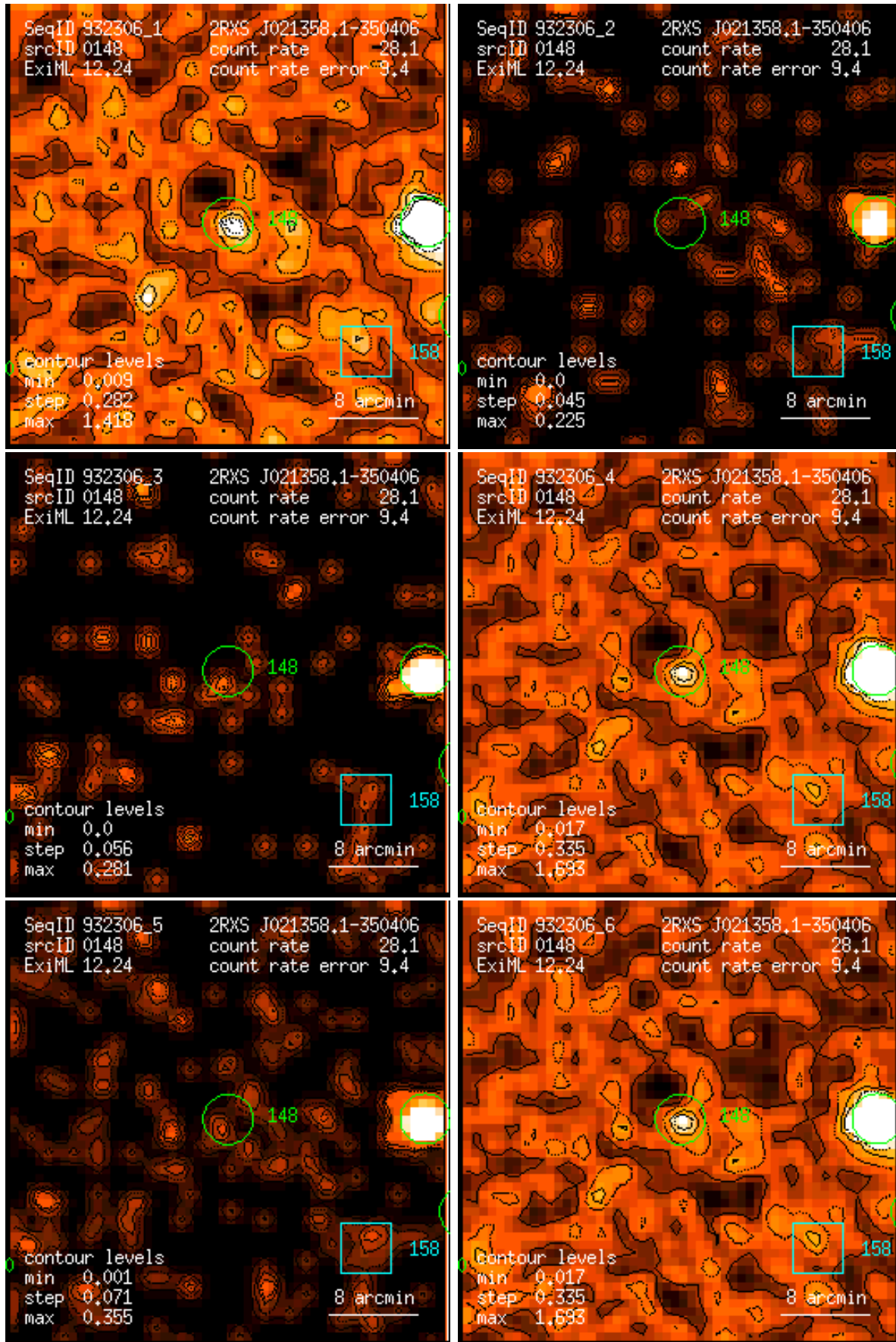
Figure 148: RASS 932306: detection 0148: band rate images, Gaussian filter: (1) PSPC channels 11 – 41, (2) 52 – 90, (3) 91 – 201, (4) 11 – 235, (5) 52 – 201, (6) 11 – 201. Broad band rates in counts/ks. Band rate contour levels in counts/ks/arcmin 2 .
