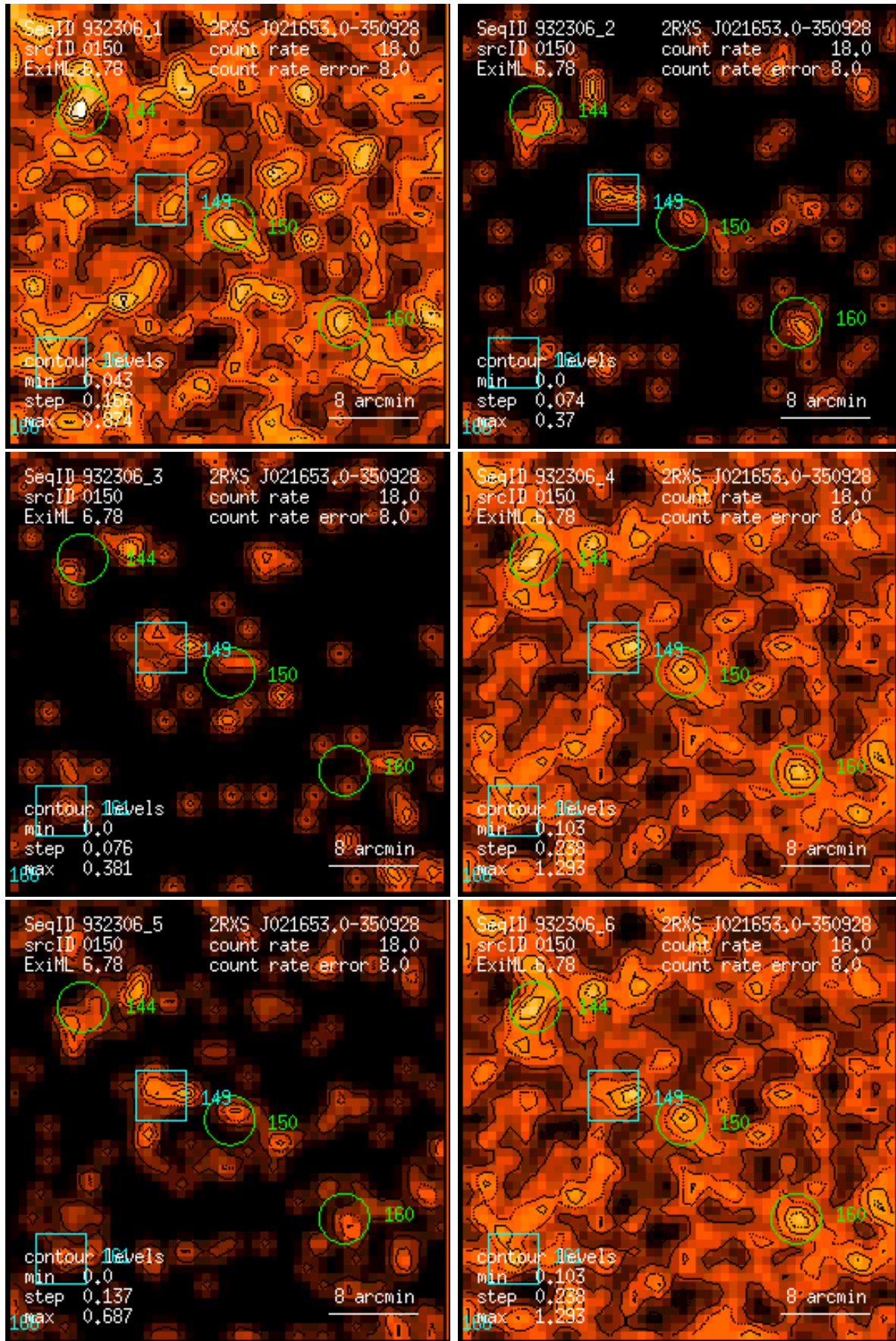
Figure 150: RASS 932306: detection 0150: band rate images, Gaussian filter: (1) PSPC channels 11 – 41, (2) 52 – 90, (3) 91 – 201, (4) 11 – 235, (5) 52 – 201, (6) 11 – 201. Broad band rates in counts/ks. Band rate contour levels in counts/ks/arcmin 2 .
