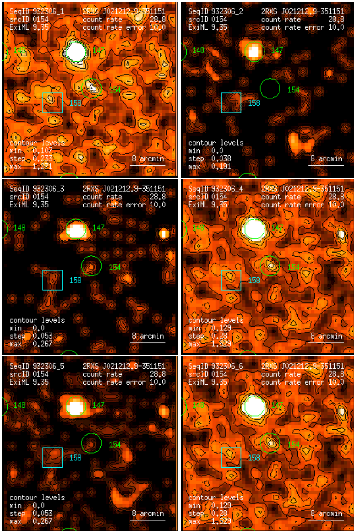
Figure 154: RASS 932306: detection 0154: band rate images, Gaussian filter: (1) PSPC channels 11 – 41, (2) 52 – 90, (3) 91 – 201, (4) 11 – 235, (5) 52 – 201, (6) 11 – 201. Broad band rates in counts/ks. Band rate contour levels in counts/ks/arcmin 2 .
