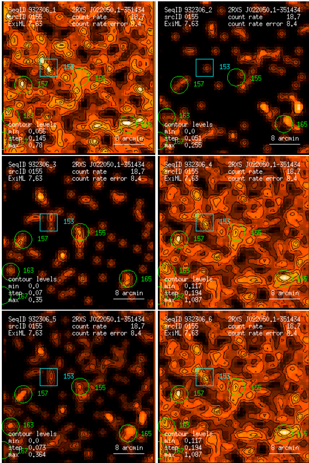
Figure 155: RASS 932306: detection 0155: band rate images, Gaussian filter: (1) PSPC channels 11 – 41, (2) 52 – 90, (3) 91 – 201, (4) 11 – 235, (5) 52 – 201, (6) 11 – 201. Broad band rates in counts/ks. Band rate contour levels in counts/ks/arcmin 2 .
