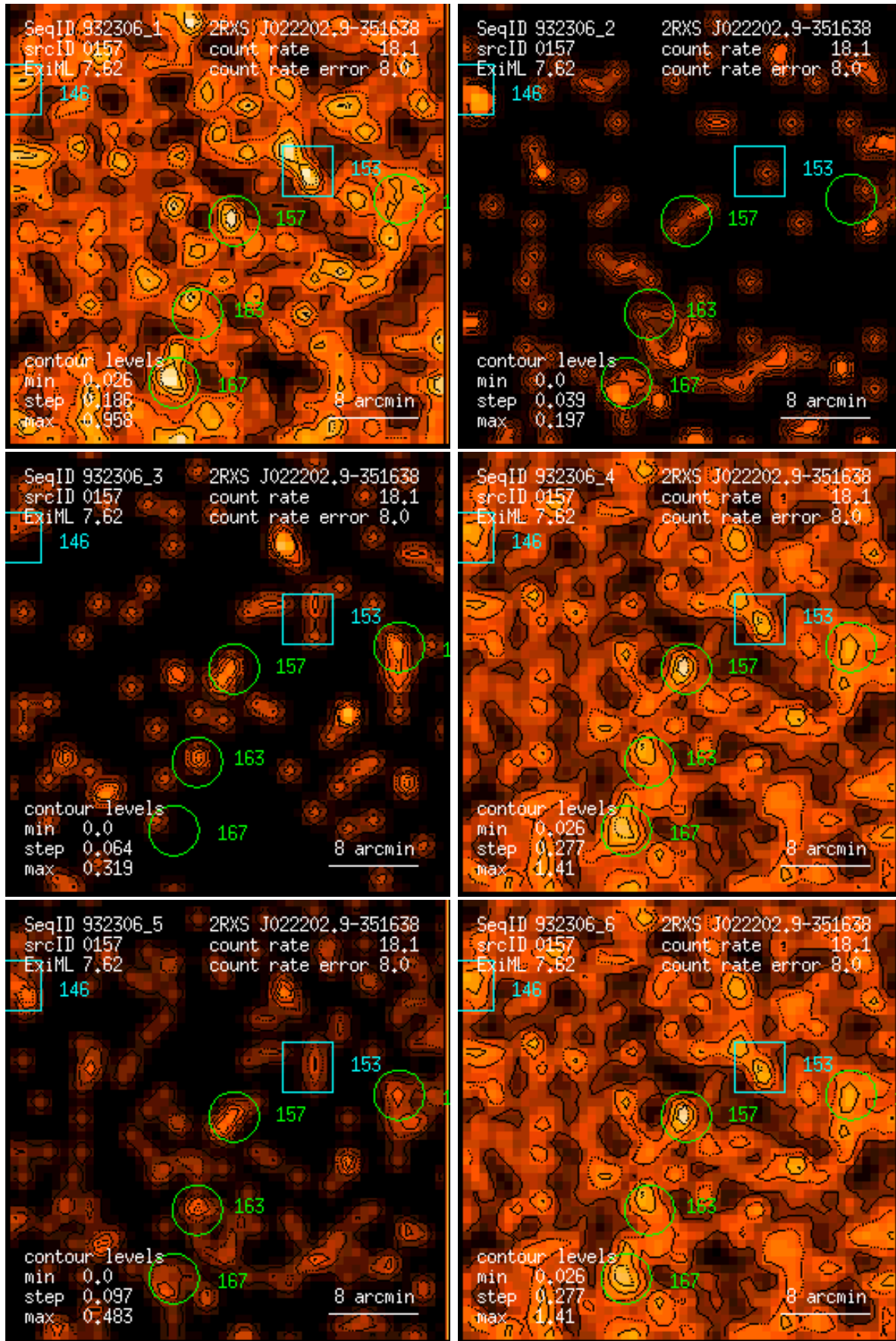
Figure 157: RASS 932306: detection 0157: band rate images, Gaussian filter: (1) PSPC channels 11 – 41, (2) 52 – 90, (3) 91 – 201, (4) 11 – 235, (5) 52 – 201, (6) 11 – 201. Broad band rates in counts/ks. Band rate contour levels in counts/ks/arcmin 2 .
