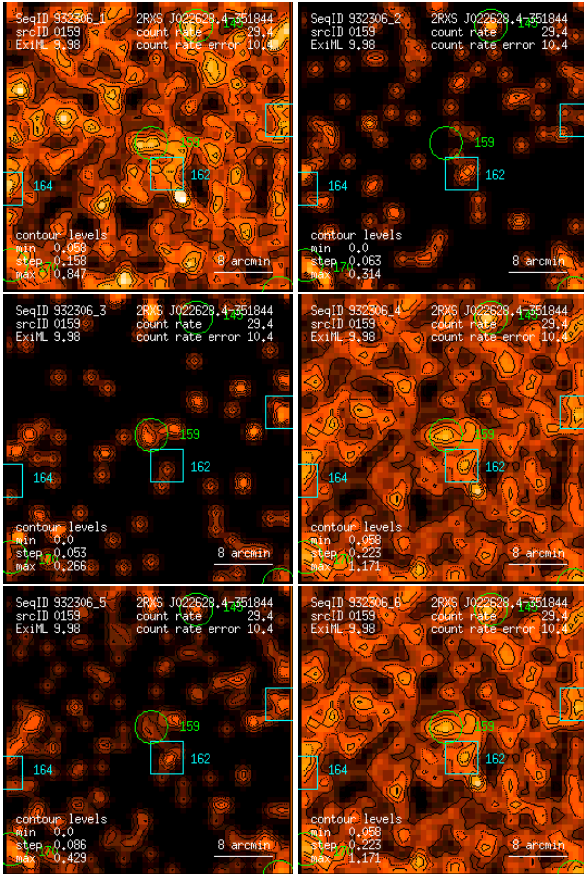
Figure 159: RASS 932306: detection 0159: band rate images, Gaussian filter: (1) PSPC channels 11 – 41, (2) 52 – 90, (3) 91 – 201, (4) 11 – 235, (5) 52 – 201, (6) 11 – 201. Broad band rates in counts/ks. Band rate contour levels in counts/ks/arcmin 2 .
