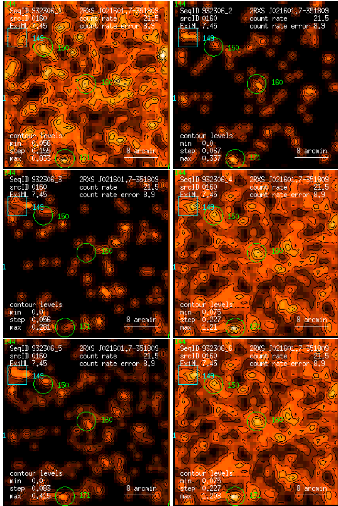
Figure 160: RASS 932306: detection 0160: band rate images, Gaussian filter: (1) PSPC channels 11 – 41, (2) 52 – 90, (3) 91 – 201, (4) 11 – 235, (5) 52 – 201, (6) 11 – 201. Broad band rates in counts/ks. Band rate contour levels in counts/ks/arcmin 2 .
