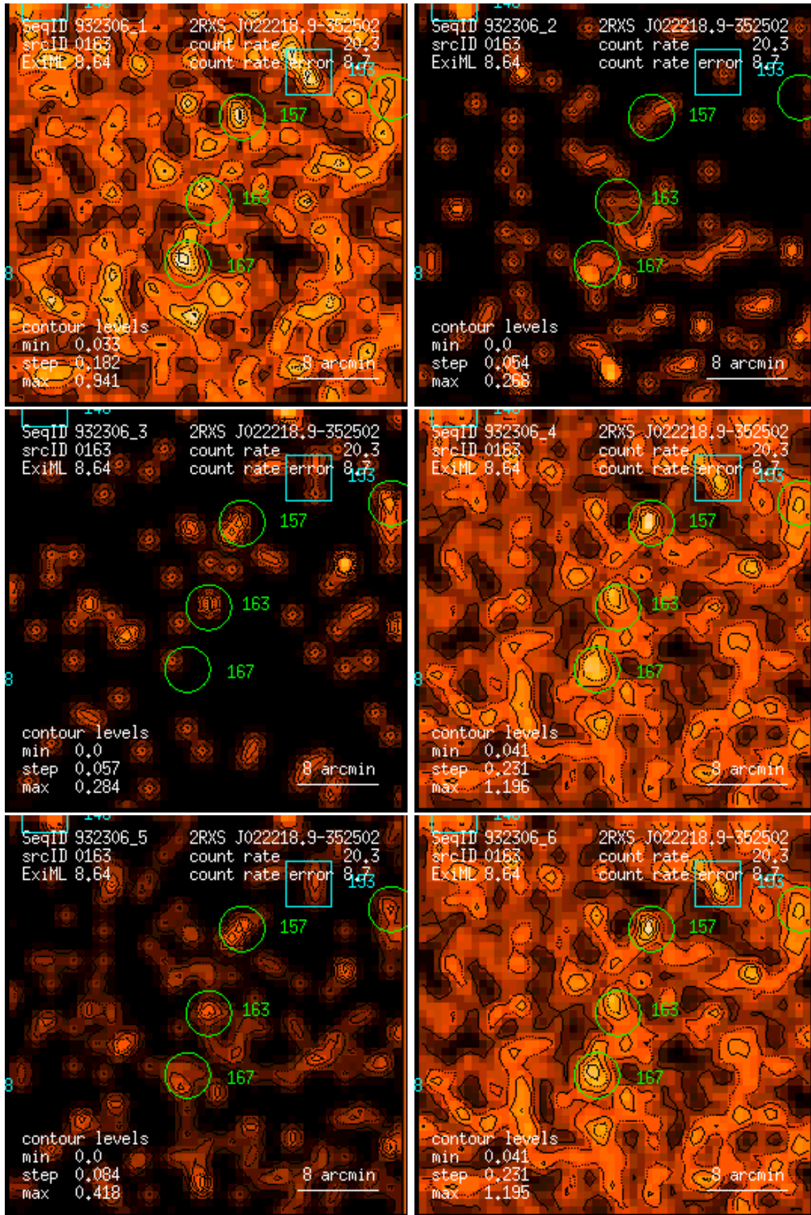
Figure 163: RASS 932306: detection 0163: band rate images, Gaussian filter: (1) PSPC channels 11 – 41, (2) 52 – 90, (3) 91 – 201, (4) 11 – 235, (5) 52 – 201, (6) 11 – 201. Broad band rates in counts/ks. Band rate contour levels in counts/ks/arcmin 2 .
