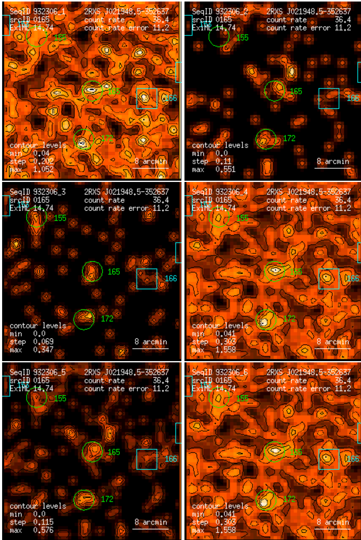
Figure 165: RASS 932306: detection 0165: band rate images, Gaussian filter: (1) PSPC channels 11 – 41, (2) 52 – 90, (3) 91 – 201, (4) 11 – 235, (5) 52 – 201, (6) 11 – 201. Broad band rates in counts/ks. Band rate contour levels in counts/ks/arcmin 2 .
