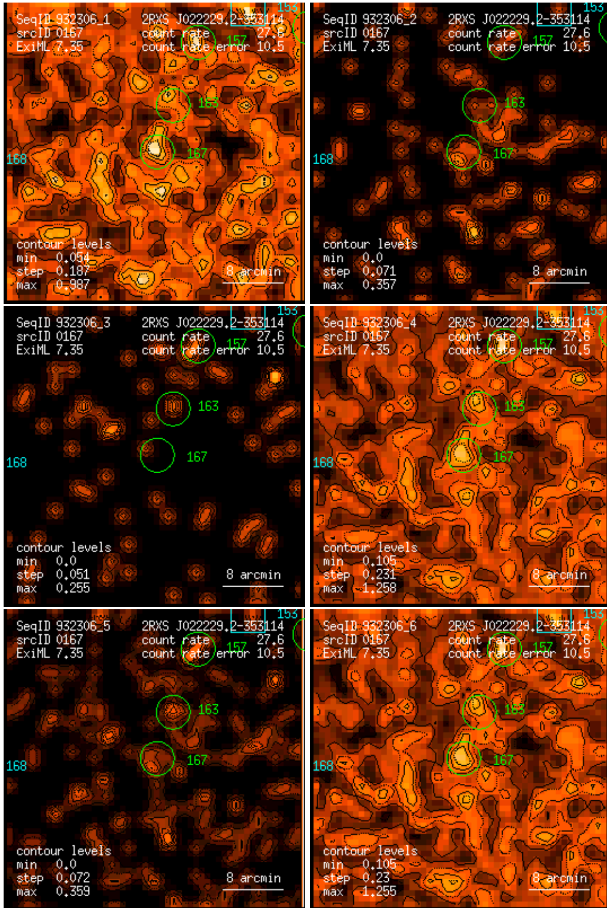
Figure 167: RASS 932306: detection 0167: band rate images, Gaussian filter: (1) PSPC channels 11 – 41, (2) 52 – 90, (3) 91 – 201, (4) 11 – 235, (5) 52 – 201, (6) 11 – 201. Broad band rates in counts/ks. Band rate contour levels in counts/ks/arcmin 2 .
