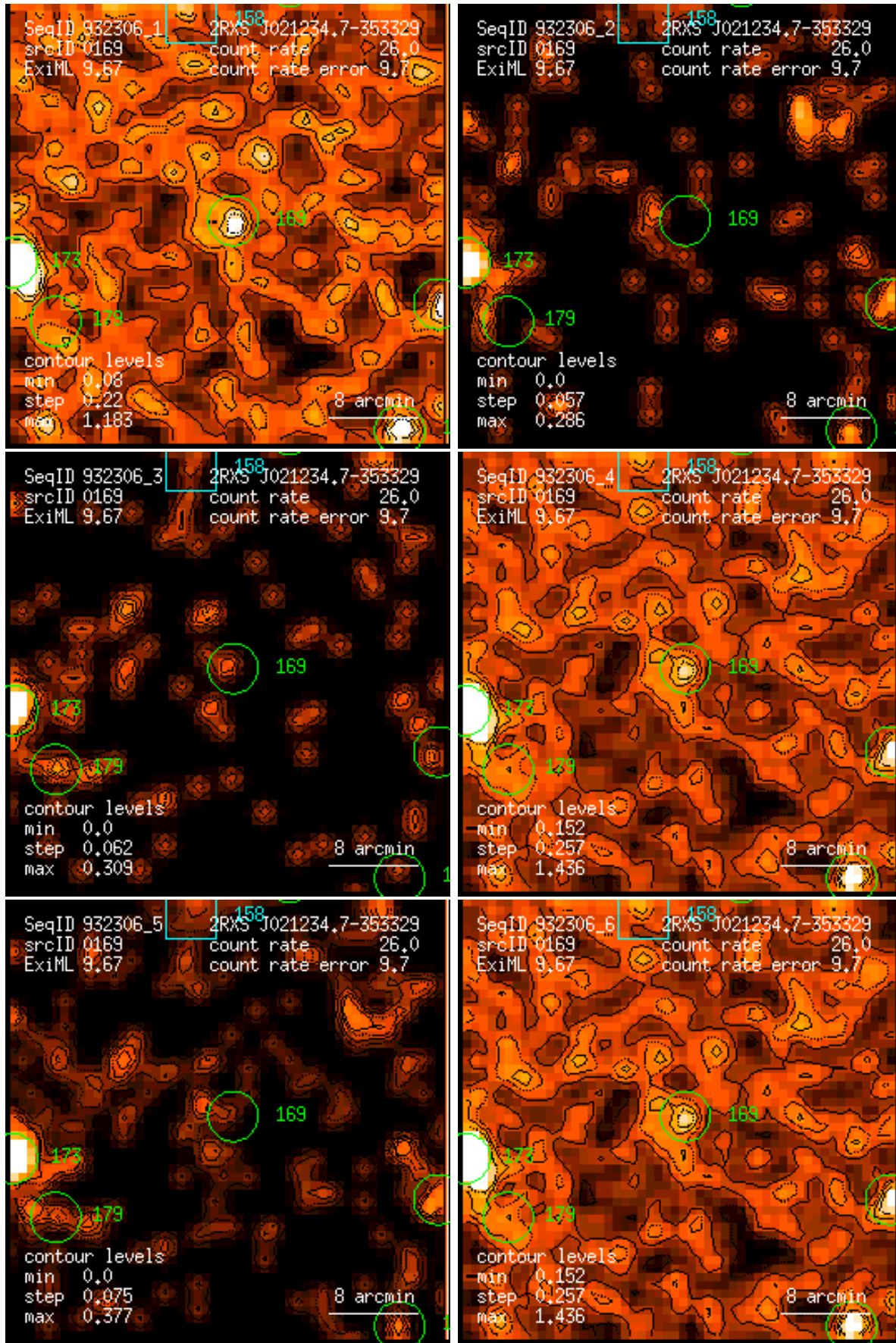
Figure 169: RASS 932306: detection 0169: band rate images, Gaussian filter: (1) PSPC channels 11 – 41, (2) 52 – 90, (3) 91 – 201, (4) 11 – 235, (5) 52 – 201, (6) 11 – 201. Broad band rates in counts/ks. Band rate contour levels in counts/ks/arcmin 2 .
