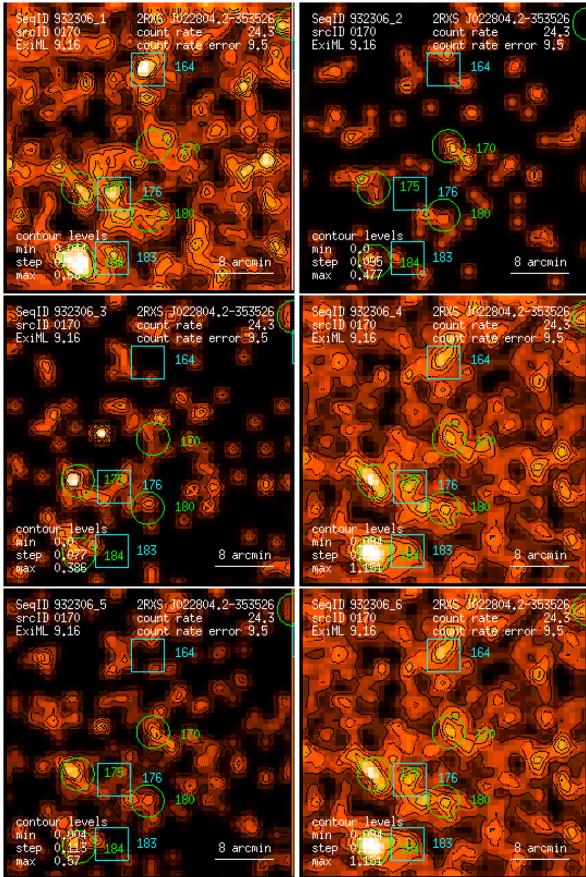
Figure 170: RASS 932306: detection 0170: band rate images, Gaussian filter: (1) PSPC channels 11 – 41, (2) 52 – 90, (3) 91 – 201, (4) 11 – 235, (5) 52 – 201, (6) 11 – 201. Broad band rates in counts/ks. Band rate contour levels in counts/ks/arcmin 2 .
