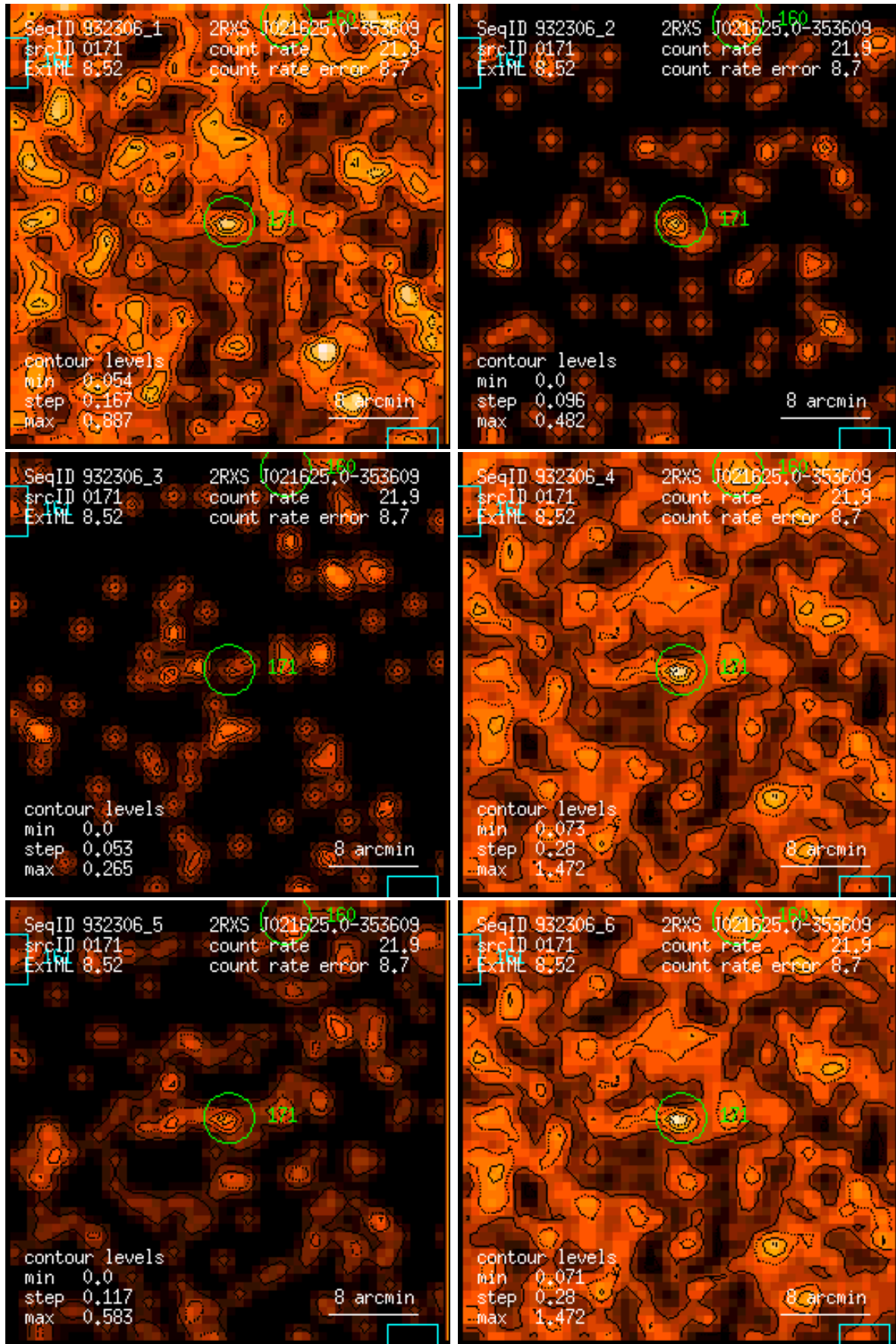
Figure 171: RASS 932306: detection 0171: band rate images, Gaussian filter: (1) PSPC channels 11 – 41, (2) 52 – 90, (3) 91 – 201, (4) 11 – 235, (5) 52 – 201, (6) 11 – 201. Broad band rates in counts/ks. Band rate contour levels in counts/ks/arcmin 2 .
