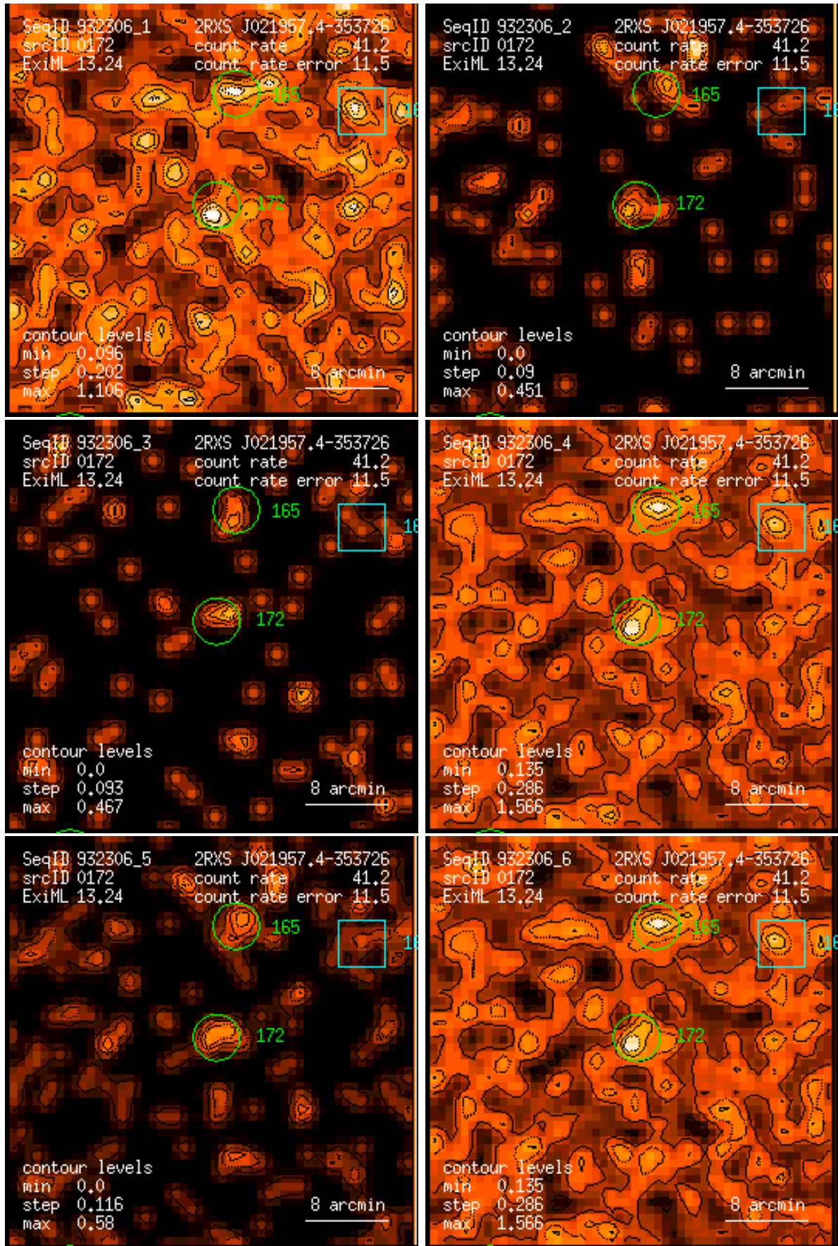
Figure 172: RASS 932306: detection 0172: band rate images, Gaussian filter: (1) PSPC channels 11 – 41, (2) 52 – 90, (3) 91 – 201, (4) 11 – 235, (5) 52 – 201, (6) 11 – 201. Broad band rates in counts/ks. Band rate contour levels in counts/ks/arcmin 2 .
