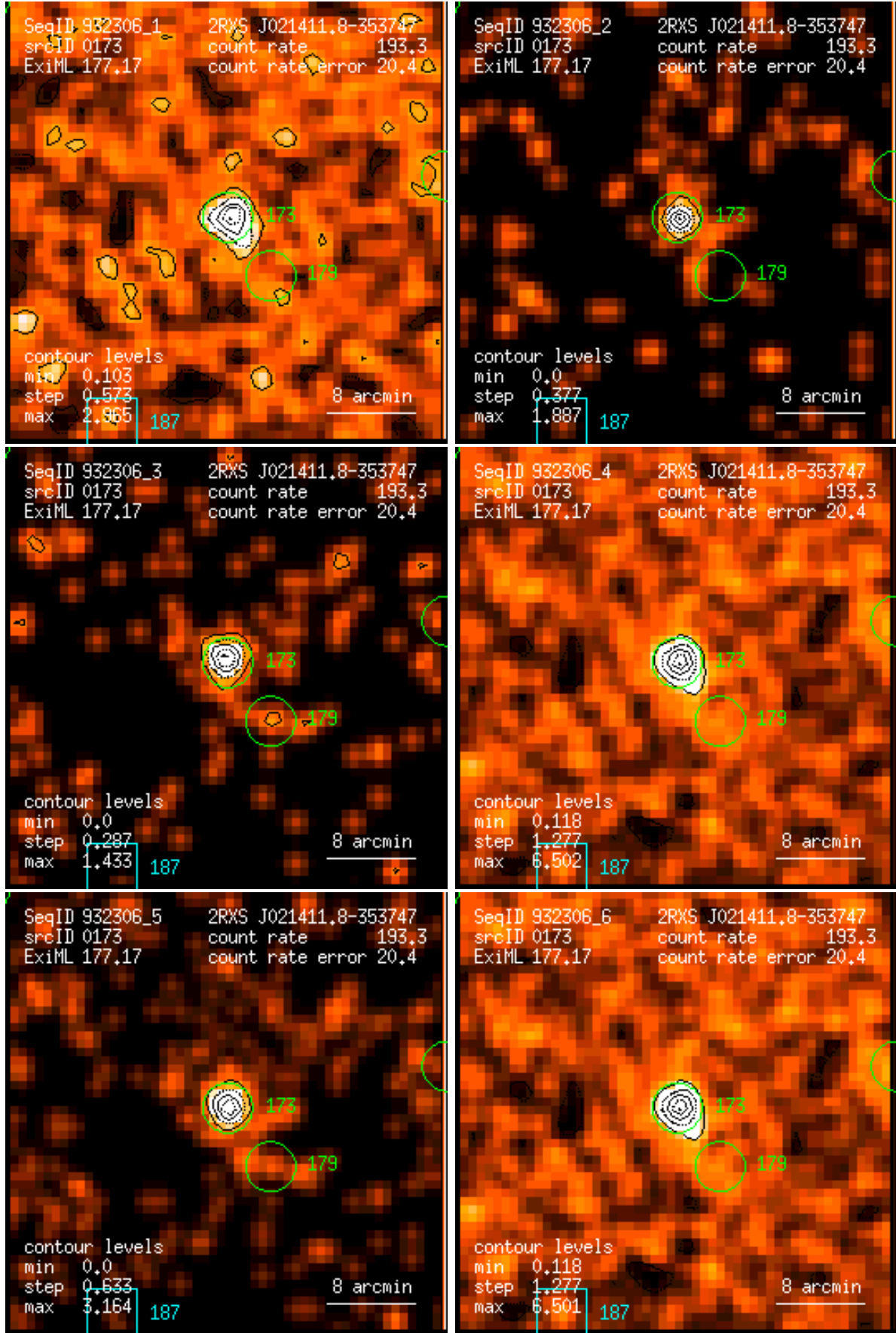
Figure 173: RASS 932306: detection 0173: band rate images, Gaussian filter: (1) PSPC channels 11 – 41, (2) 52 – 90, (3) 91 – 201, (4) 11 – 235, (5) 52 – 201, (6) 11 – 201. Broad band rates in counts/ks. Band rate contour levels in counts/ks/arcmin 2 .
