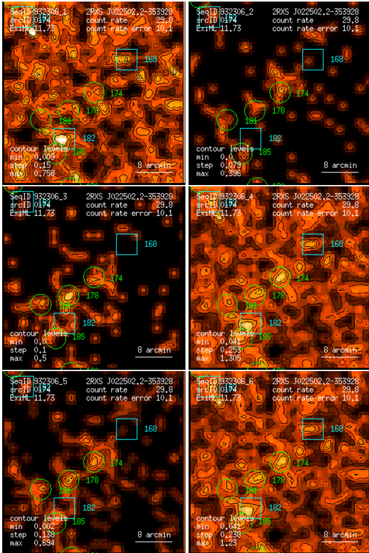
Figure 174: RASS 932306: detection 0174: band rate images, Gaussian filter: (1) PSPC channels 11 – 41, (2) 52 – 90, (3) 91 – 201, (4) 11 – 235, (5) 52 – 201, (6) 11 – 201. Broad band rates in counts/ks. Band rate contour levels in counts/ks/arcmin 2 .
