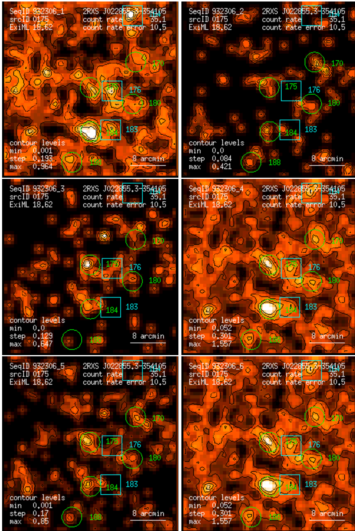
Figure 175: RASS 932306: detection 0175: band rate images, Gaussian filter: (1) PSPC channels 11 – 41, (2) 52 – 90, (3) 91 – 201, (4) 11 – 235, (5) 52 – 201, (6) 11 – 201. Broad band rates in counts/ks. Band rate contour levels in counts/ks/arcmin 2 .
