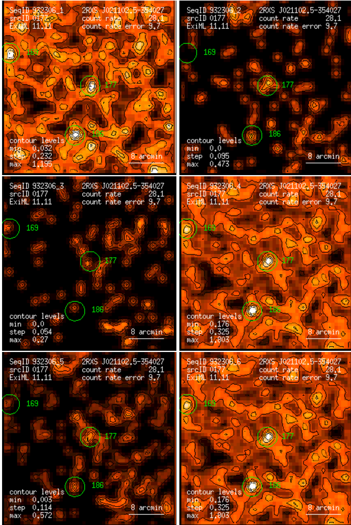
Figure 177: RASS 932306: detection 0177: band rate images, Gaussian filter: (1) PSPC channels 11 – 41, (2) 52 – 90, (3) 91 – 201, (4) 11 – 235, (5) 52 – 201, (6) 11 – 201. Broad band rates in counts/ks. Band rate contour levels in counts/ks/arcmin 2 .
