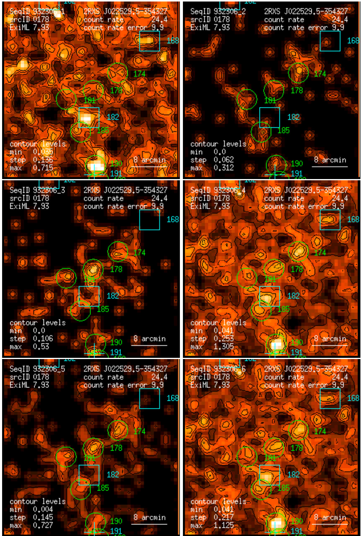
Figure 178: RASS 932306: detection 0178: band rate images, Gaussian filter: (1) PSPC channels 11 – 41, (2) 52 – 90, (3) 91 – 201, (4) 11 – 235, (5) 52 – 201, (6) 11 – 201. Broad band rates in counts/ks. Band rate contour levels in counts/ks/arcmin 2 .
