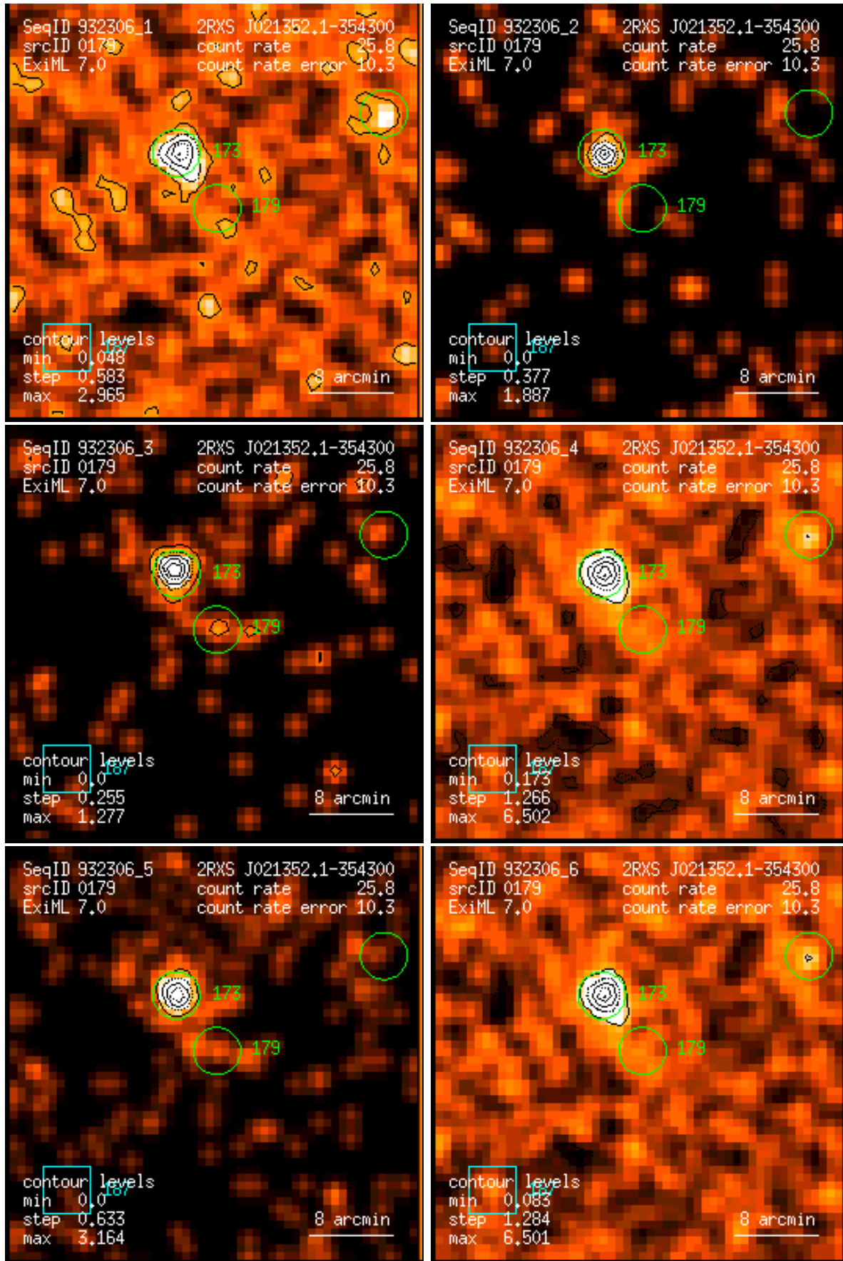
Figure 179: RASS 932306: detection 0179: band rate images, Gaussian filter: (1) PSPC channels 11 – 41, (2) 52 – 90, (3) 91 – 201, (4) 11 – 235, (5) 52 – 201, (6) 11 – 201. Broad band rates in counts/ks. Band rate contour levels in counts/ks/arcmin 2 .
